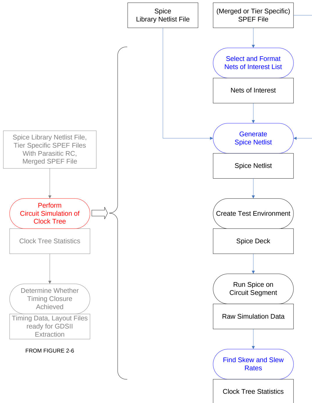
Figure 3-1: Simulation Based Timing Verification Flow
