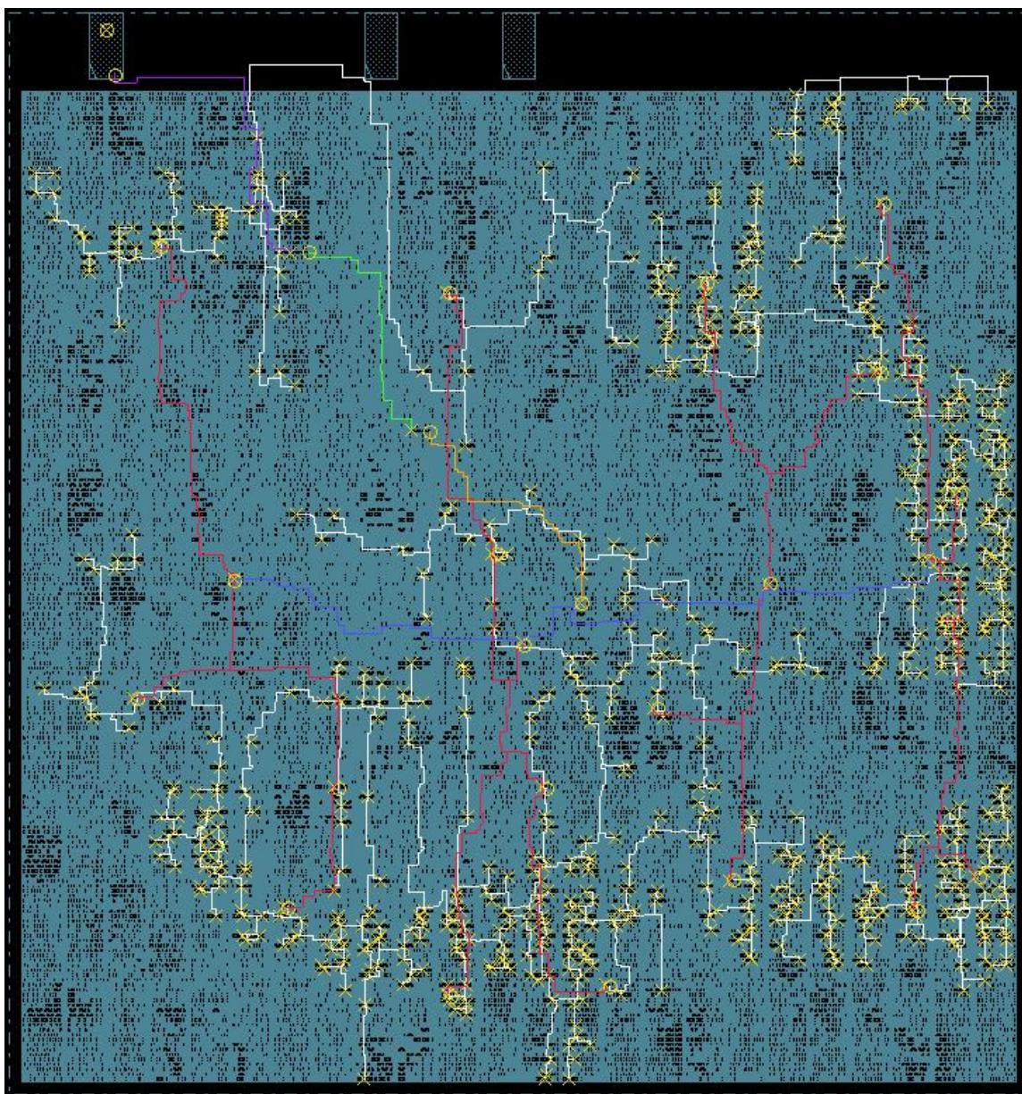
Figure 5-2: FFT Tier B Clock Tree
