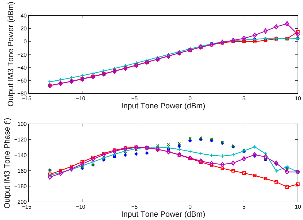
Figure 7.10: Measured and estimated magnitude and phase of Hittite amplifier IM3 products using various fitting techniques to extract the one-slice model, (* - IM3L measured, × - IM3H measured, □ - two-tone fit to a_3 and a_5 , + - nonlinear optimization fit to both data sets, ◇ - GA fit to both data sets.)
