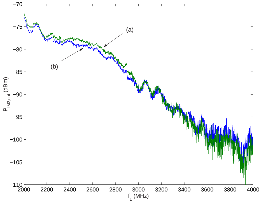
Figure 6.3: Measured output power of (a) IM3H and (b) IM3L at -15 \text{ dBm} input tone power.
