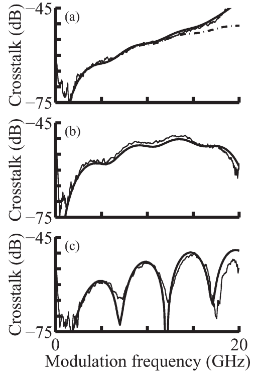
Fig. 2. Comparison between theory and experimental measurement of crosstalk for a link with dispersion-compensating fiber at the end. The dispersion-compensating fiber was cut to lengths corresponding to (a) 0%, (b) 50%, and (c) 100% of the link's accumulated dispersion. The thick solid curves show the results from the theory, whereas the thin solid curves show experimental data. The dot-dashed curve in (a) shows the result of the theory when pump distortion is neglected.
