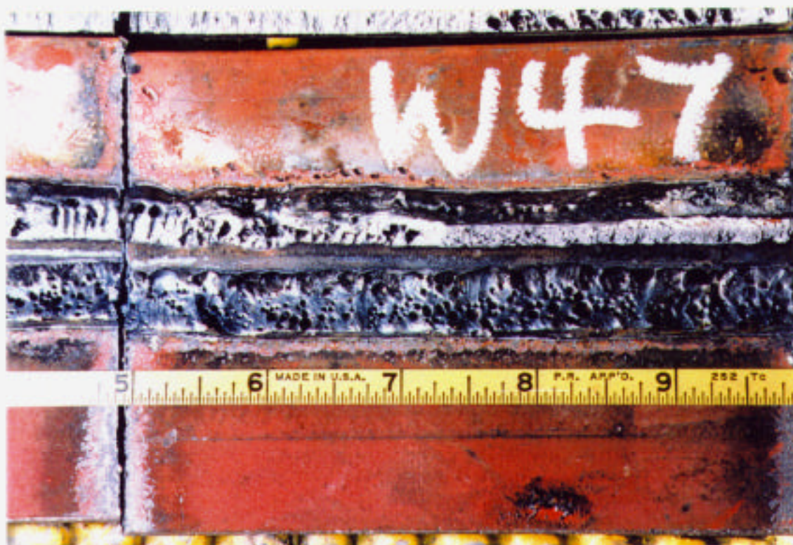
Photograph showing linear porosity along the fusion centerline of panel W47 (see Table 3-3, Devran 720).
