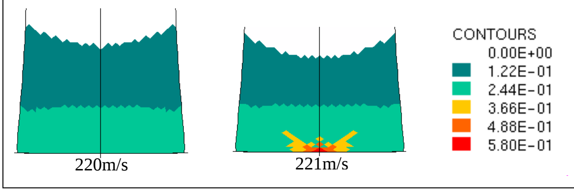
Figure 7. Predicted strain contours showing incipient strain localization in the Taylor anvil test ( t = 11 \mu s is shown; separation from the anvil occurs at about 14 \mu s ).
