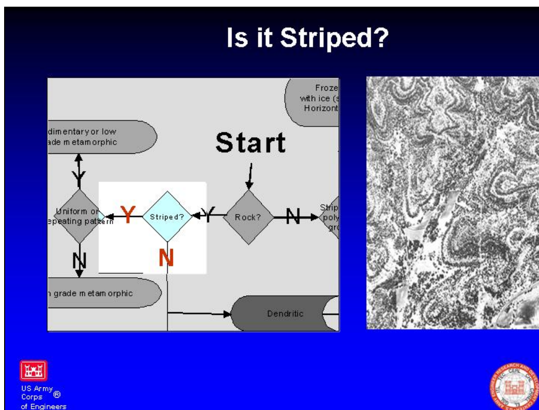
Figure 38. Illustration of the storyboard approach. The left side of the image shows the position of the user within the logic process. He has already determined that the landform polygon he is trying to classify contains rock. At this point, he is trying to determine whether or not that rock is striped. The right side of the image shows an example of striped rock provided to assist him in making this decision.
