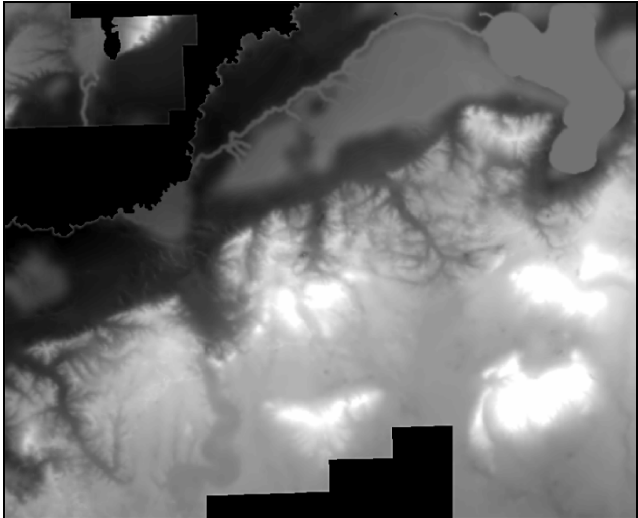
Figure 33. Depth-to-groundwater DEM.
