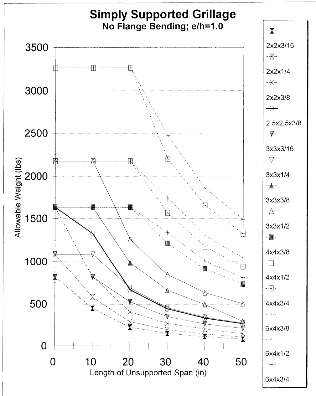
Figure 7-8 — Simply Supported Grillage, No Flange Bending; e/h = 1.0
