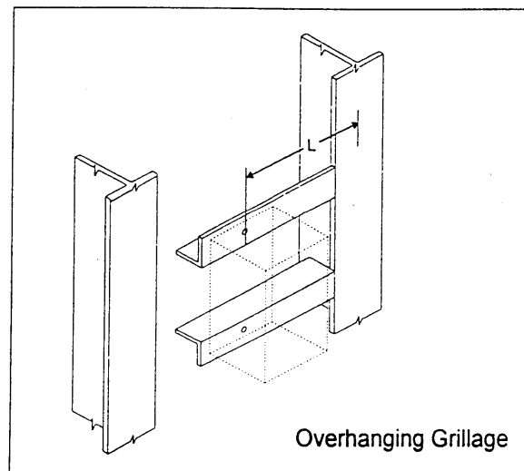
Figure 5-1 — Grillage Off-deck and Overhanging Grillage Configurations
