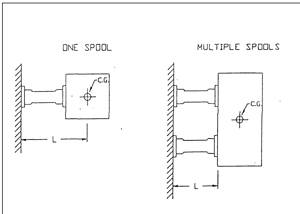
Figure 4-7 — Spool Mounted Equipment
