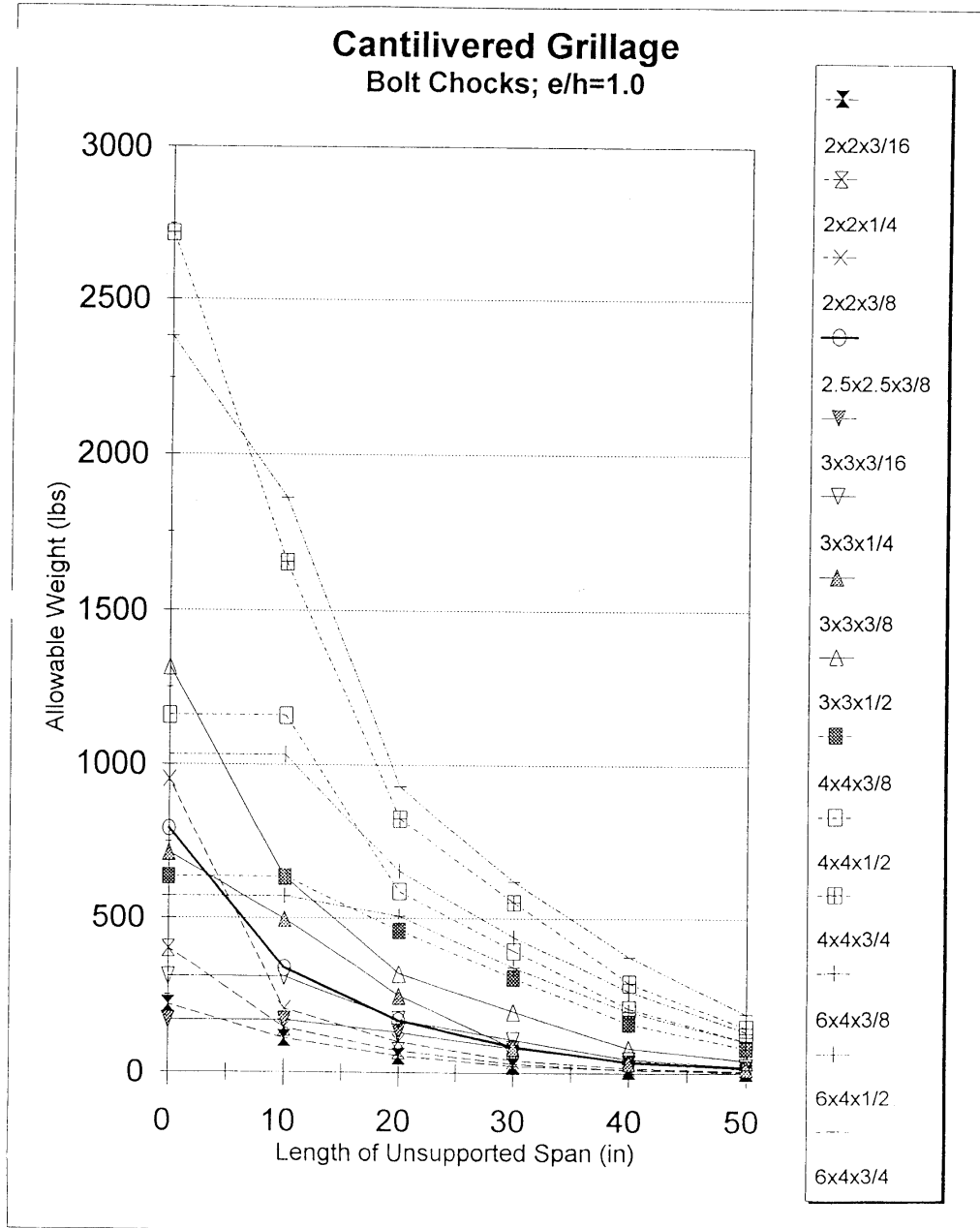
Figure 7-14 — Cantilevered Grillage, Bolt Chocks; e/h = 1.0
