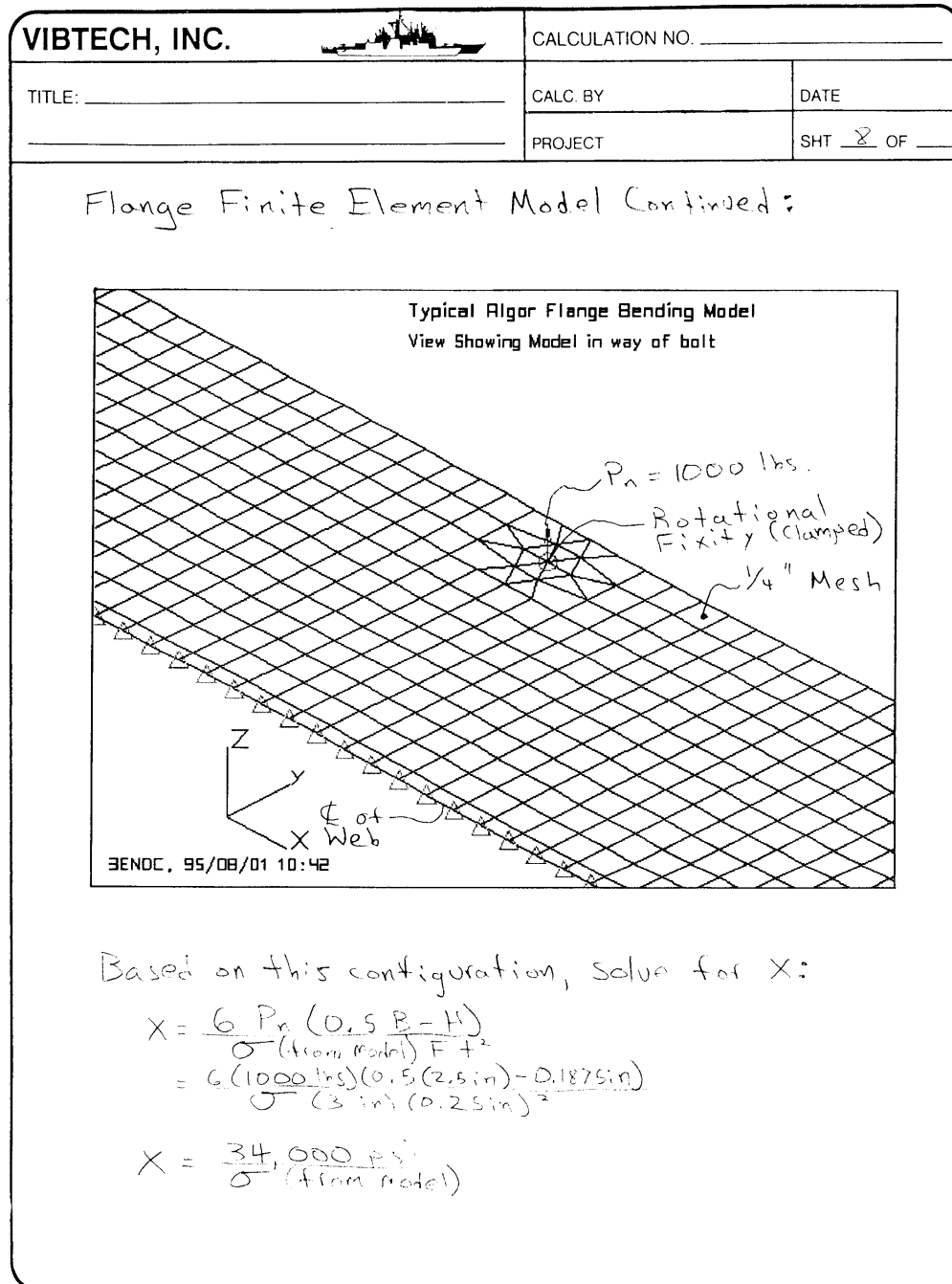
Figure 5-8 — Flange Finite Element Model (Cont'd)
