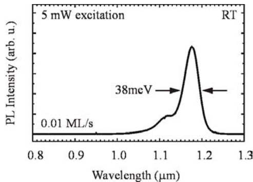
Fig. 3 PL spectrum of InAs/GaAs SA-QDs embedded in GaAs at RT
