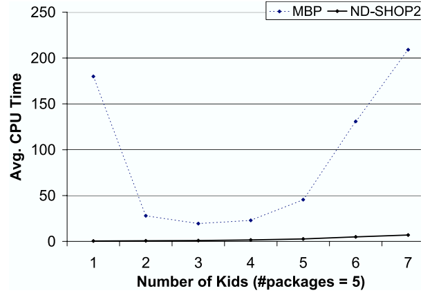
Figure 4: Average running times of ND-SHOP2 and MBP on Robot-Navigation problems, as a function of the number of kid-doors. The number of packages in the domain is fixed to 5.
