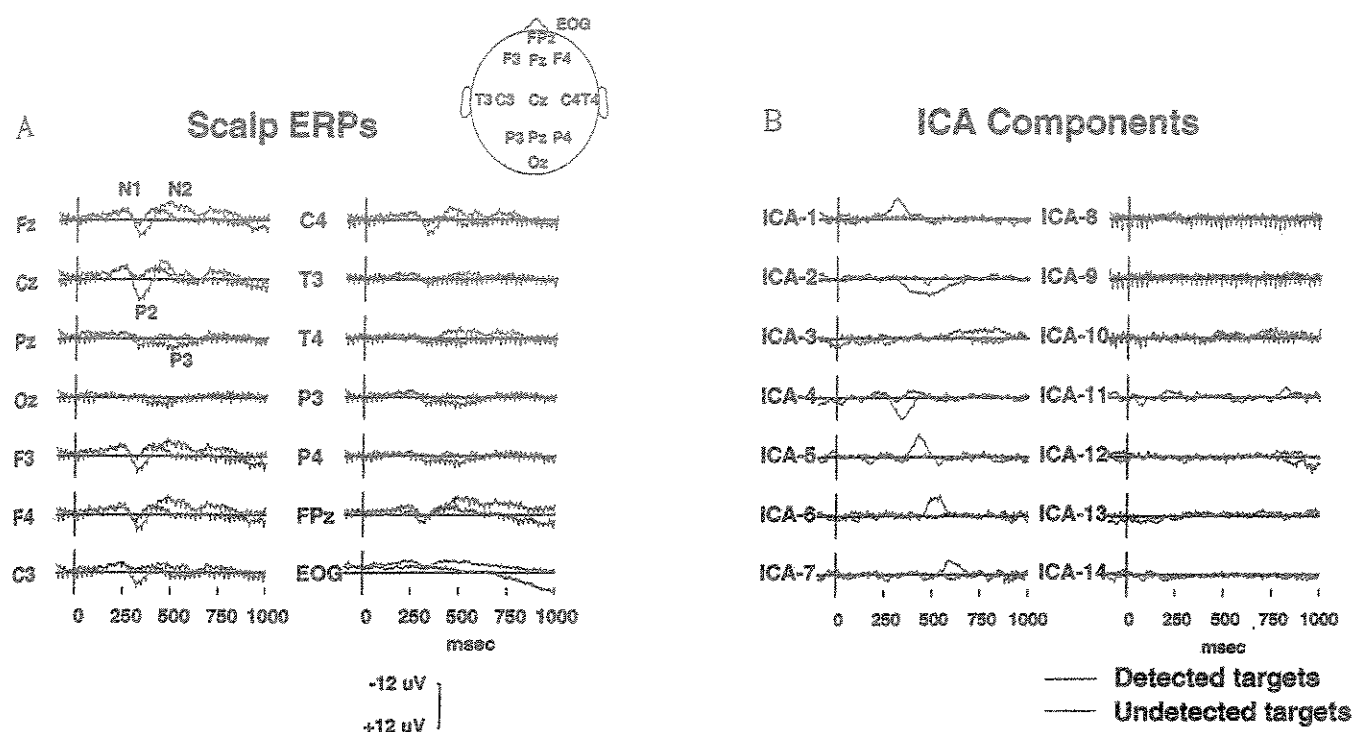
FIG. 2. Decomposition of an ERP data set. (A) Averaged evoked responses at 14 scalp channels from one subject in a sustained auditory detection experiment (23) to detected (blue traces, 209 epochs) and undetected (red traces, 81 epochs) slow-onset noise-burst targets. (B) Activation wave forms of the resulting 14 ICA components during the detected (blue traces) and undetected (red traces) response epochs. Seven components (ICA-1 to ICA-7) are predominantly activated for a period of 50–300 ms during one or the other response. Three more ICA components (ICA-8 to ICA-10) compose the auditory SSR (22) to a click train presented throughout the experiment at one-eighth the EEG sampling rate. The remaining four ICA components (ICA-11 to ICA-14) presumably sum activity of multiple weak brain and extra-brain sources.
