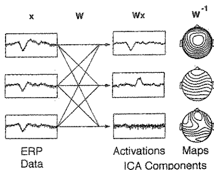
FIG. 1. Schematic overview of ICA of EEG data. (A) (Upper) Averaged (or single) EEG epochs, x , recorded from multiple scalp sites are used to train an "unmixing" weight matrix, W , so as to maximize the entropy of the nonlinearly transformed output, g(Wx) . (Lower) After training, rows of the trained weight matrix, W , are linear spatial filters decomposing the input data into the independent activities of the ICA components. Rows of the product of W and the input data, x , are the activation waveforms of the ICA components, while columns of the inverse weight matrix, W^{-1} , map their projections onto the scalp electrodes. (B) (Inset) Schematic illustration of ICA decompositions of a simulated evoked response, recorded at two electrodes (A and B), summing the activity of two temporally independent response sources (#1 and #2) with arbitrary (focal or diffuse) spatial distributions. (Upper) Scatterplot of potentials recorded at the two electrodes, showing the response as a two-dimensional trajectory. In this plot, the activity of source #1 alone would lie on the near-vertical axis ICA-1; the activity of source #2 alone would lie on the near-horizontal (but not orthogonal) axis ICA-2. If the time courses of activation of the two brain networks are independent of one another, the summed output of sources #1 and #2 will, over time, fill the dashed parallelogram. The first principal component of the data (PCA-1) indicates the direction of maximum data variance, but neither this nor the second principal component orthogonal to it identifies either of the independent components. (Lower) The ICA algorithm finds the directions of the two axes (ICA-1, ICA-2) by maximizing the entropy of the data linearly transformed to the ICA component axes and nonlinearly transformed using a logistic sigmoid. The linear transformation and sigmoidal nonlinearity rotates and spreads the data to fill the dashed square as evenly as possible, whereas in the original (A, B) space (above), the data remain within an oblique parallelogram.
