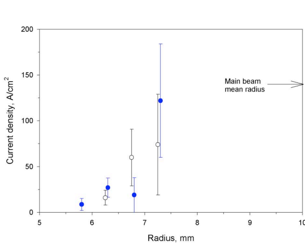
Fig. 5 Estimated current density profiles for 12 mm and 10 mm (in blue) quartz rod diameters. Measured data were obtained at \sim 280 kV accelerating voltage ( \sim 1.1 kA main beam current) and \sim 2.6 T guide magnetic
