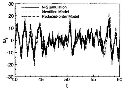
Figure 2: Vorticity fluctuations time history of Navier-Stokes simulations, identified model, and reduced-order model.
