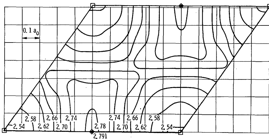
(c) \sigma/a_0 = 1.20 .
