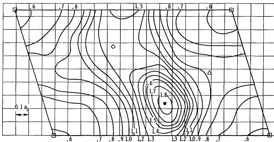
(a) \sigma/a_0 = 0.80 .
