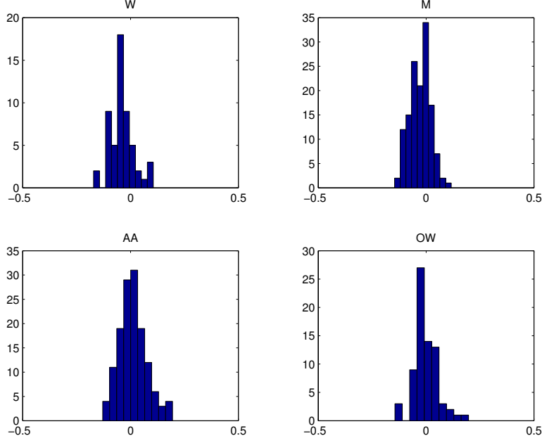
Figure 7-1: Histograms for the \alpha_1 parameter for the \backslash w \backslash , \backslash m \backslash , \backslash aa \backslash and \backslash ow \backslash phones.
