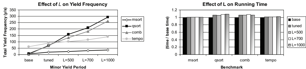
Figure 9.3: Effect of L on Yielding Performance ( Y=100M , E=100 , H=50 )
