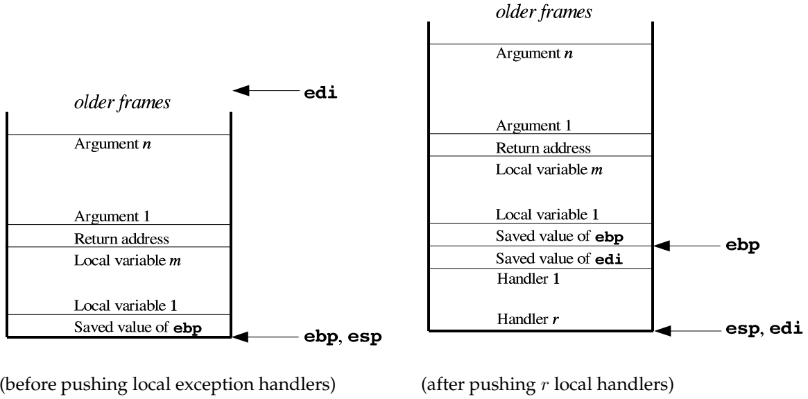
Figure 7.4: A Lilt function's stack frame
