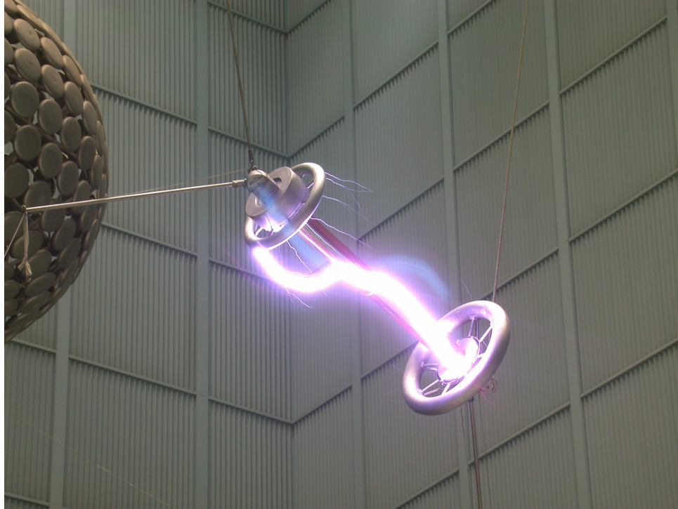
Figure 16. Cutler insulator at Hydro Quebec showing partial surface flashover.
