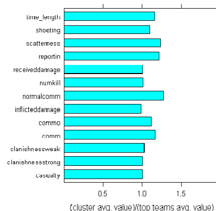
Communication Cluster 1
