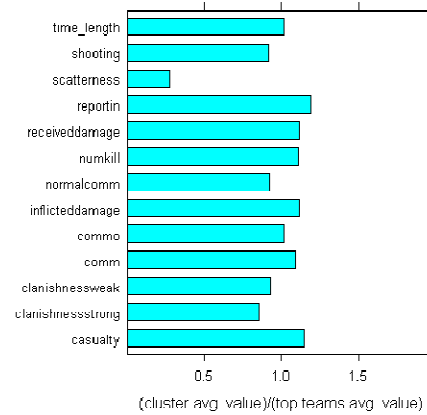
Movement Cluster 5
