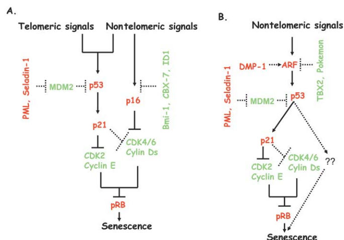
Figure 2. Telomeric and nontelomeric signals induce senescence via tumor suppressor pathways in human and mouse cells
