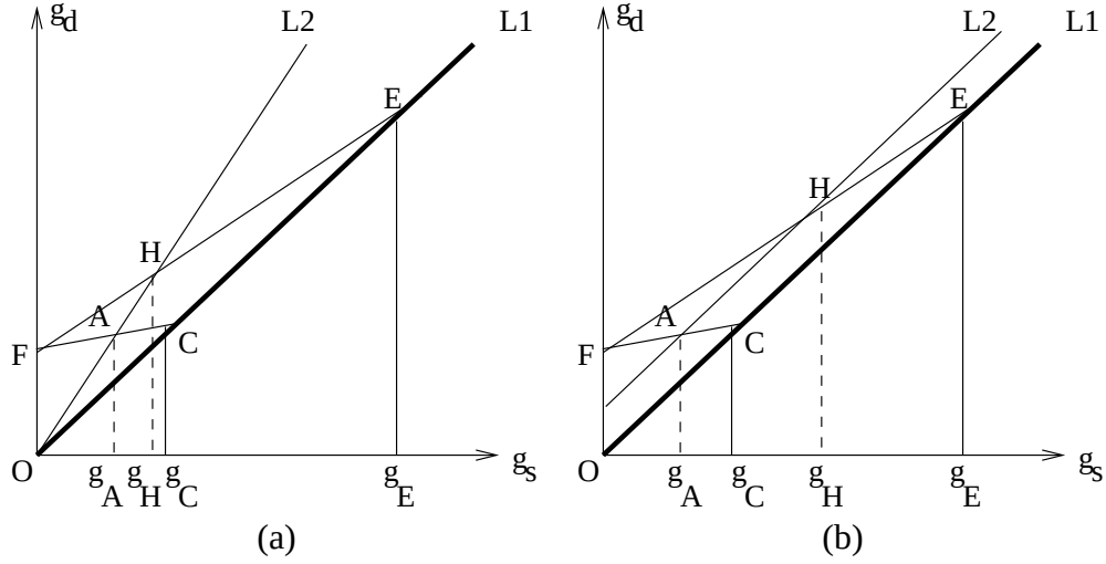
Figure 2.19: The performance of using different turning-point detection formula
