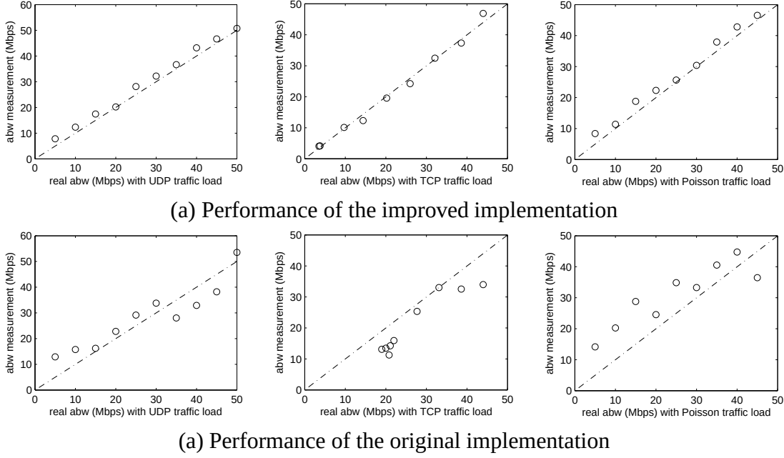
Figure 2.20: Performance of the improved IGI/PTR implementation
