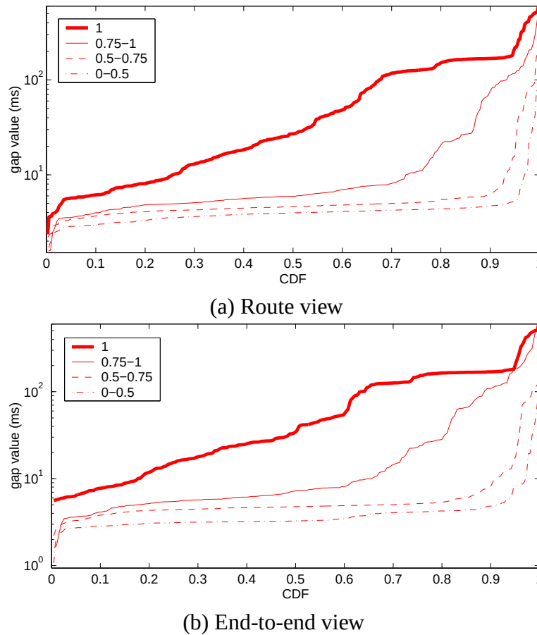
Figure 4.7: Bottleneck gap value vs. bottleneck persistence
