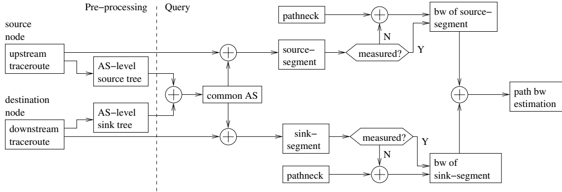
Figure 6.2: BRoute System Architecture
