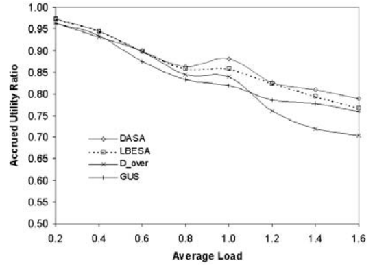
Fig. 9. Algorithm AUR's: Step TUF's, No Dependencies, and Exponential Distributions
