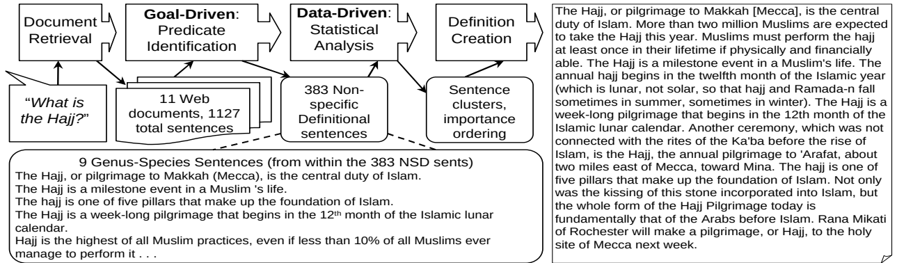
Figure 1: DefScriber answers “What is the Hajj?”
