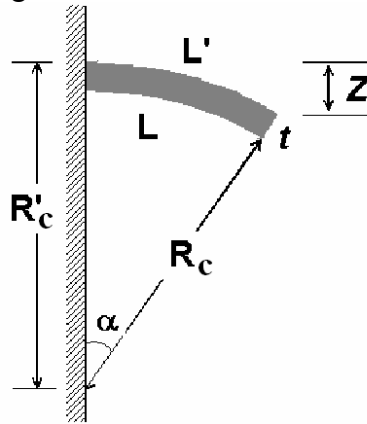
Figure 30: Schematic representation of side and front view of a rectangular microcantilever
