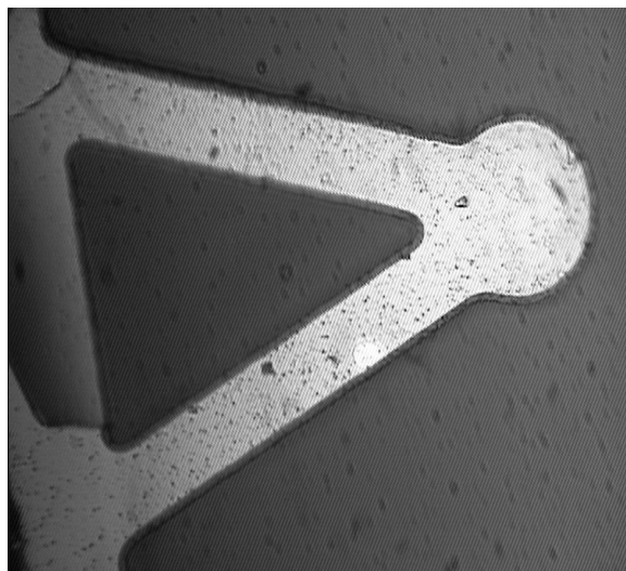
Figure 34. The optical microscope pictures of microcantilever surfaces after five LbL treatments by the hydrogel microspheres (Magnification \times 750).
