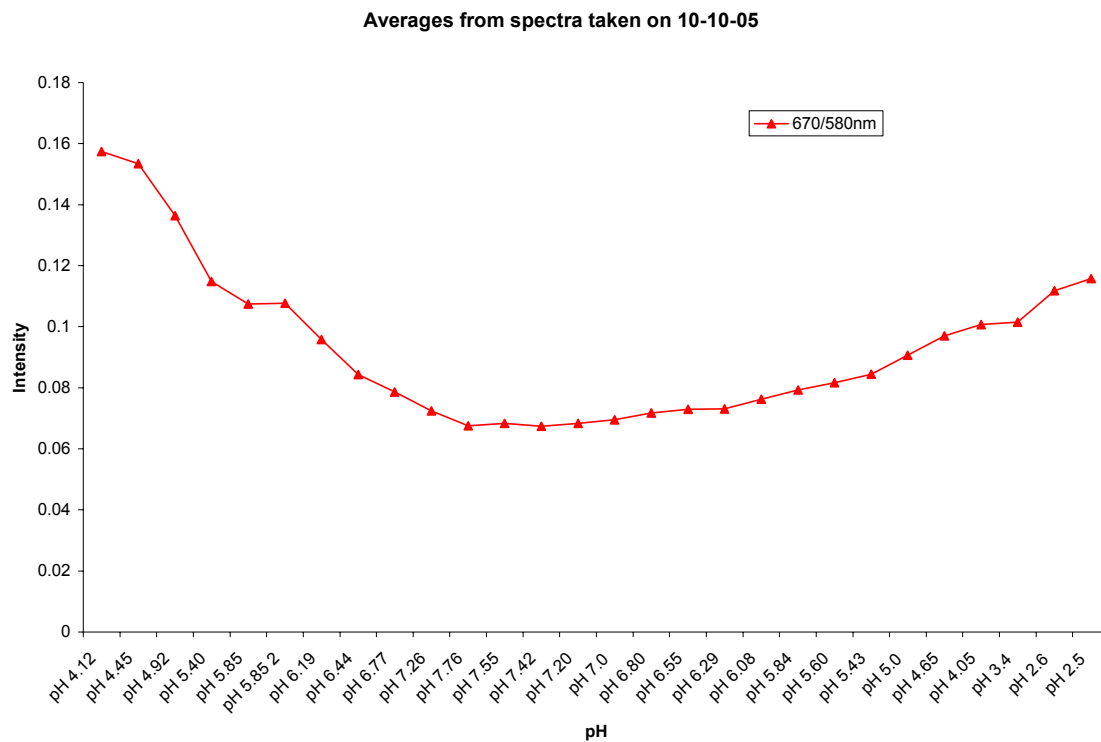
Figure 26: Ratio Value vs. pH for TRITC/AF647-Labeled Poly(AA-co-AM) Particles
