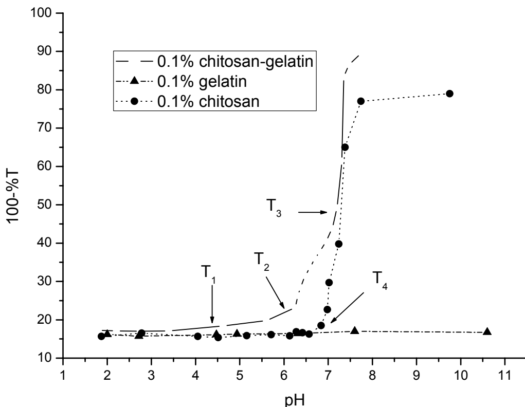
Figure 18: Turbidity titration curves of gelatin, chitosan and gelatin/chitosan mixture solutions at 420nm
