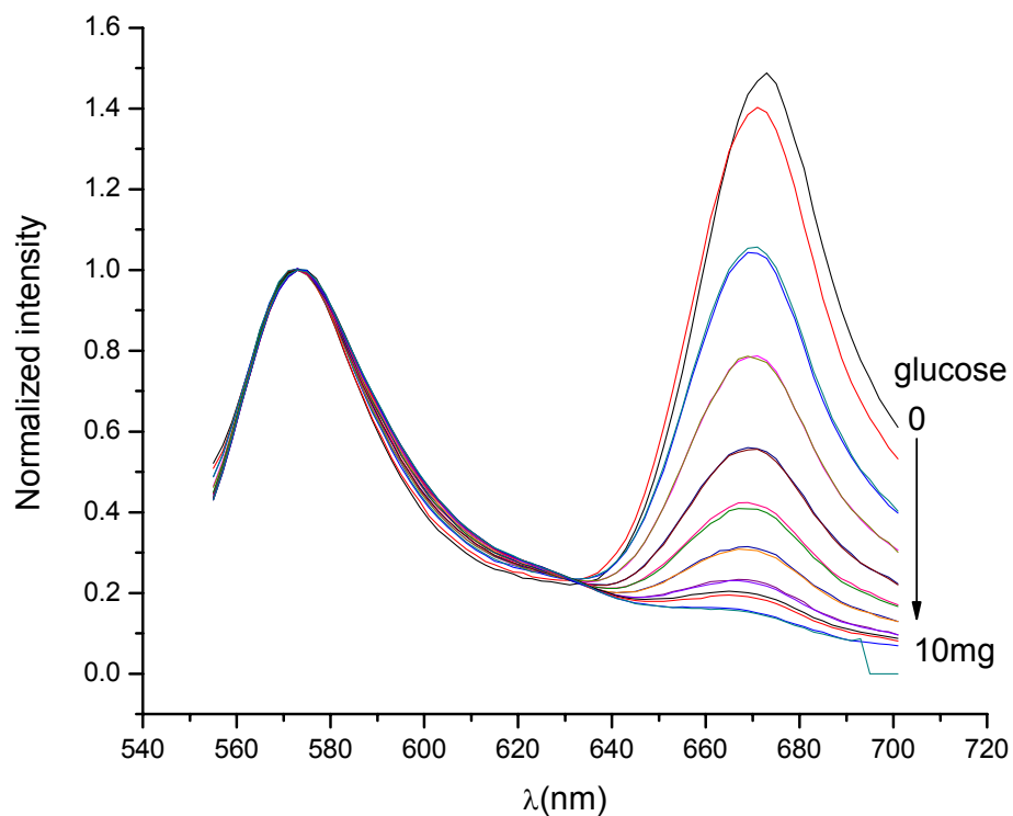
Figure 55: Change in the normalized fluorescent spectra of GOx loaded TRITC and Alexa Fluor 647™-labeled chitosan/gelatin microspheres with the titration of glucose into deionized water. (Ex=543nm, Em=555-700nm)
