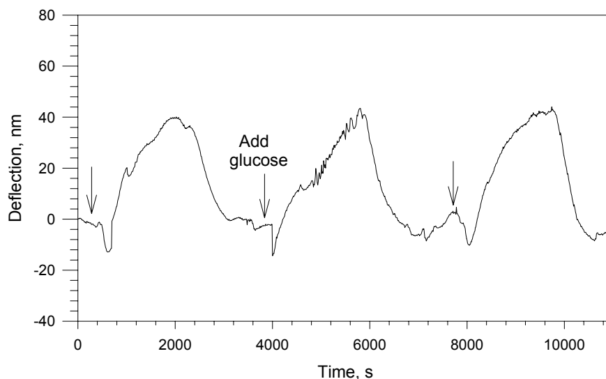
Figure 27: Three replications of the bending response as a function of time following injection of a solution of 2mM glucose in 0.01M NaCl solution (the injection points are indicated with arrows). The silicon microcantilever was coated with a 15 \mu m thick GOx-doped poly(acrylamide) hydrogel.
