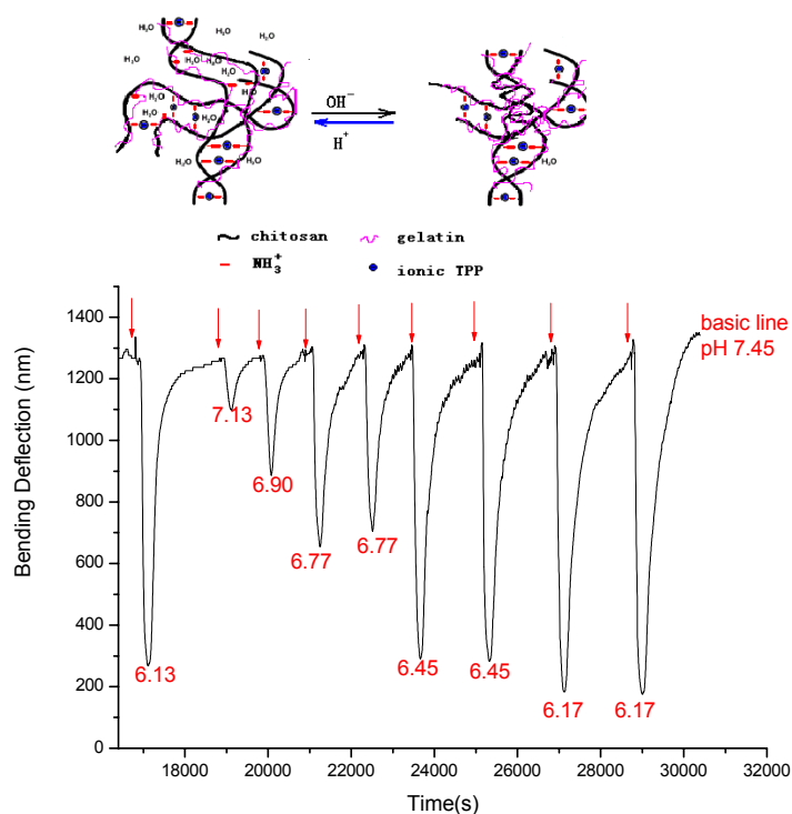
Figure 23: Steady bending response as a function of time for chitosan/gelatin gel (C:G=1:1, 3.5% TPP at pH=6.0) coated microcantilever, upon injection of a 0.1M PBS at various pH. The injection time is indicated with arrows.
