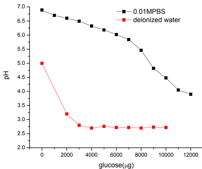
Figure 60: Comparison of the changes in external pH with the titration of glucose into deionized water and 0.01M PBS.
