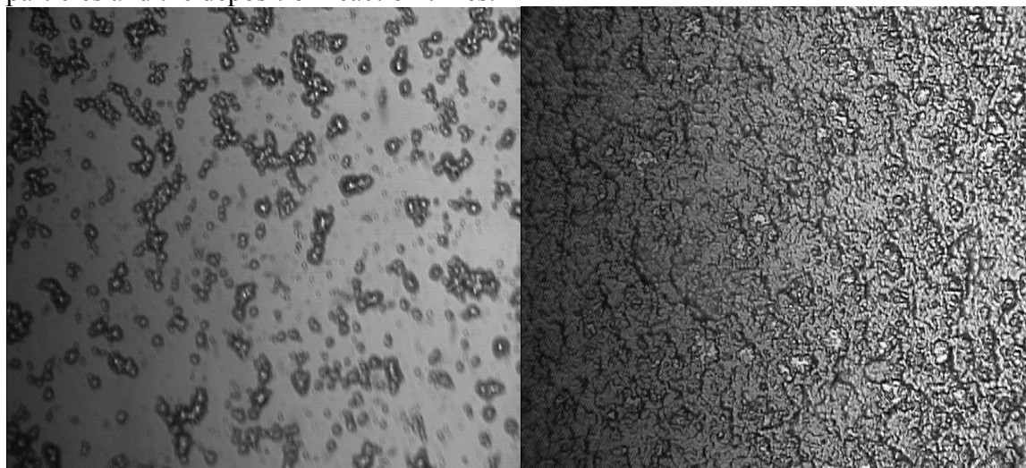
Figure 33. The optical microscope pictures of wafer surfaces after first (Left) and 5 (Right) adsorption cycles involving the hydrogel microspheres (Magnification \times 750).
