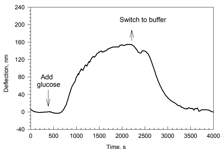
Figure 20: Bending response as a function of time for a silicon microcantilever coated with a 15 \mu m thick layer of GOx-doped hydrogel upon injection of a concentration of 8mM glucose solutions in 0.01M NaCl background electrolyte solution
