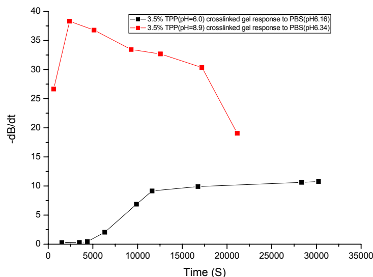
Figure 24: The speed of the bending response (-dB/dt) of the chitosan/gelatin hydrogel crosslinked by 3.5% TPP at pH 6.0 and 8.9
