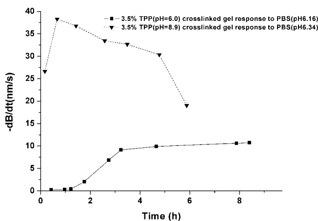
Figure 6. Maximum bending rate ( -dB/dt ) of cantilevers modified with chitosan/gelatin hydrogel crosslinked by 3.5% TPP at pH 6.0 and 8.9. Each data point is a separate deflection rate measurement in response to addition of pH 6 PBS to a cantilever (baseline of pH 7.4 PBS).
