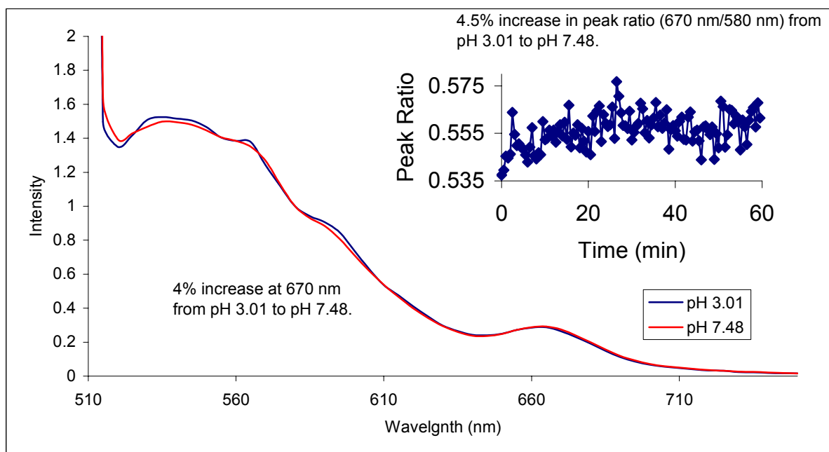
Figure 105. Transient pH response of microspheres (0.1% glutaraldehyde) from pH 3.01 to pH 7.48.
