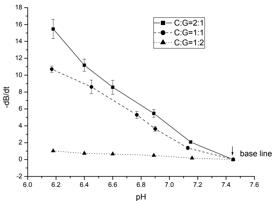
Figure 25: The steady response speed ( -dB/dt ) of chitosan/gelatin with different ratio of C:G (crosslinked with 3.5% TPP pH=6.0) coated on the microcantilever as a function of pH (Experiments were run in triplicate per sample. All data were expressed as means \pm standard deviation (SD) for n=3 ).
