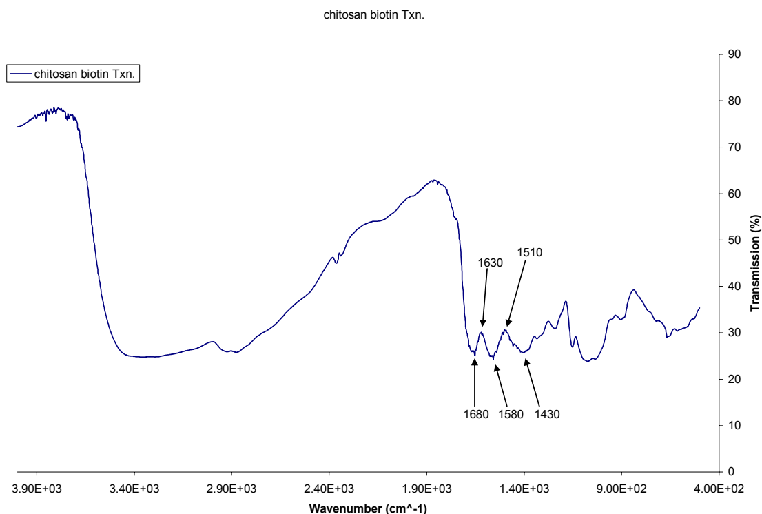
Figure 13. Infrared spectrum of biotinylated chitosan.
