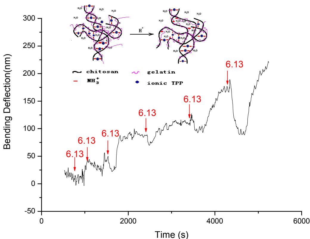
Figure 22: The transient bending response as a function of time for chitosan/gelatin gel (C:G=1:1, 3.5% TPP at pH=6.0) coated microcantilever, upon injection of a 0.01M PBS at pH 6.13, basic line was 0.01M PBS pH 7.45. The injection time is indicated with arrows.
