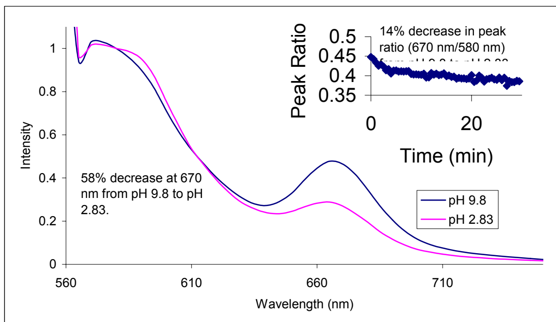
Figure 106. Transient pH response of microspheres (0.1% glutaraldehyde) from pH 9.8 to pH 2.83.
