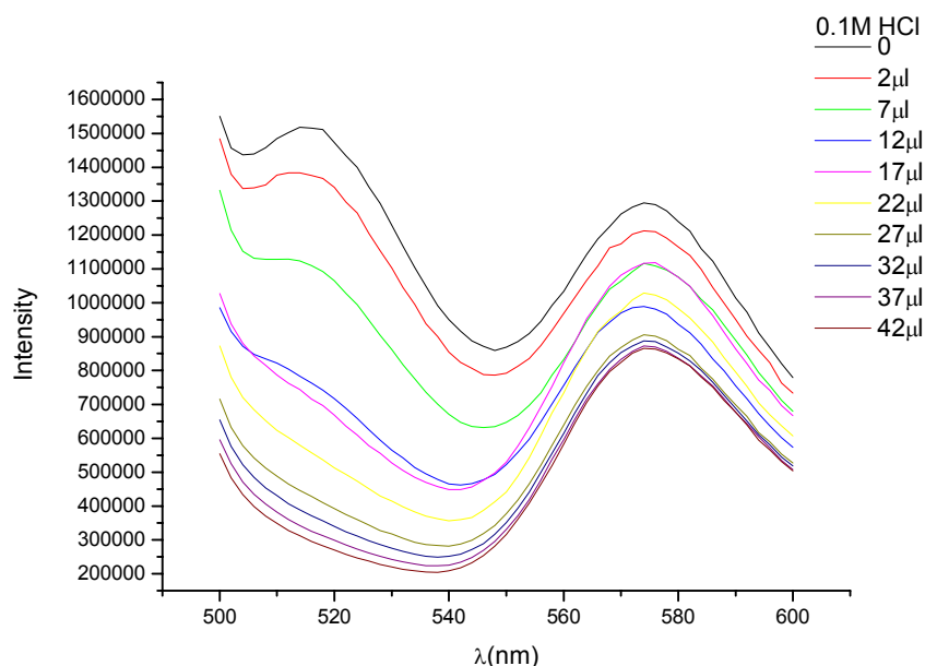
Figure 49: The fluorescent spectra of FITC and TRITC dual-labeled chitosan/gelatin microspheres, while different volume of 0.1M HCl was added into the solution to change the pH.
