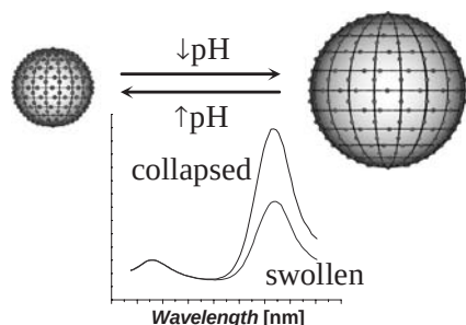
Figure 1. Schematic of the smart sensor operation based on RET transduction of pH-sensitive swelling. Drawings illustrate the sensor structure and relative positions of fluorophores, and the corresponding spectra match the energy transfer of the system to the volume changes.
