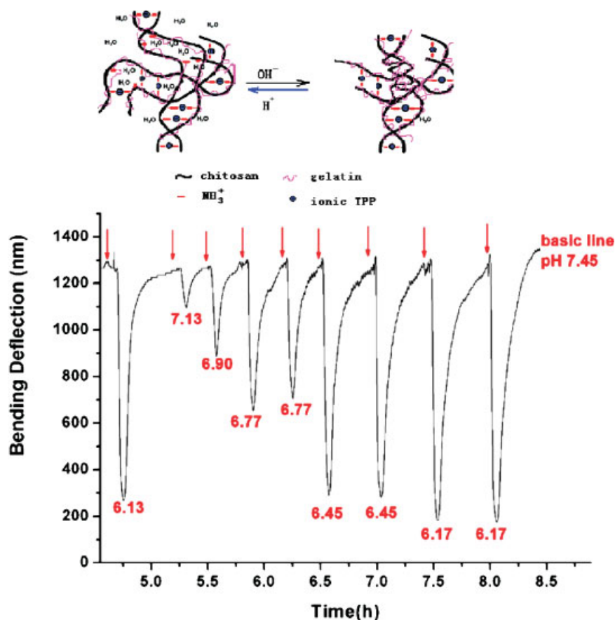
Figure 5. Steady-state (preconditioned) bending response versus time for chitosan/gelatin (C:G = 1:1, 3.5% TPP at pH = 6.0) gel-coated microcantilever, upon injection of a 0.1M PBS at various pH. Injection times are indicated with arrows.
