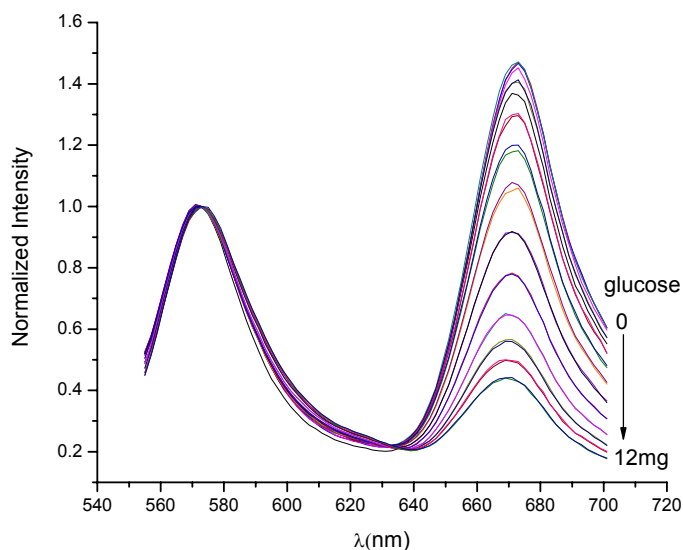
Figure 57: Change in the normalized fluorescent spectra of GOx loaded TRITC and Alexa Fluor 647 TM labeled chitosan/gelatin microspheres with the titration of glucose into 0.01MPBS. (Ex=543nm, Em=555-700nm)
