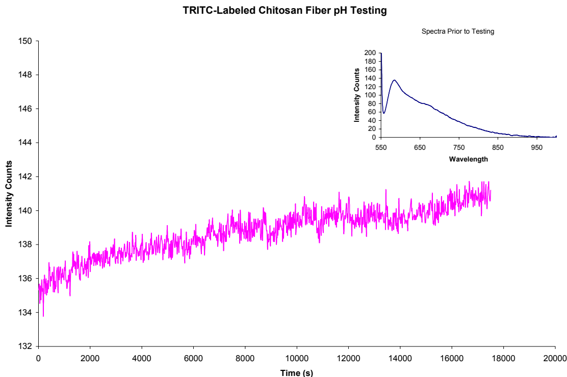
Figure 70: Response of TRITC-Labeled Chitosan Hydrogel to Changes in pH
