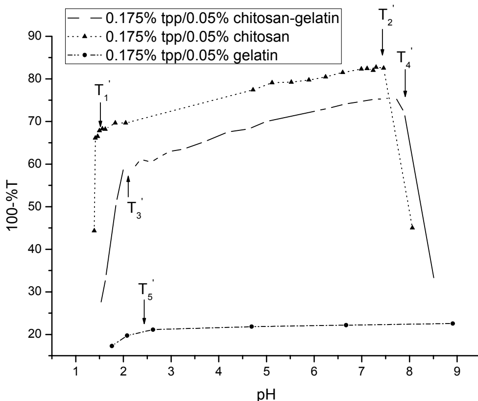
Figure 19: Turbidity titration curves of TPP/gelatin, TPP/chitosan and TPP/gelatin/chitosan mixture solutions at 420nm
