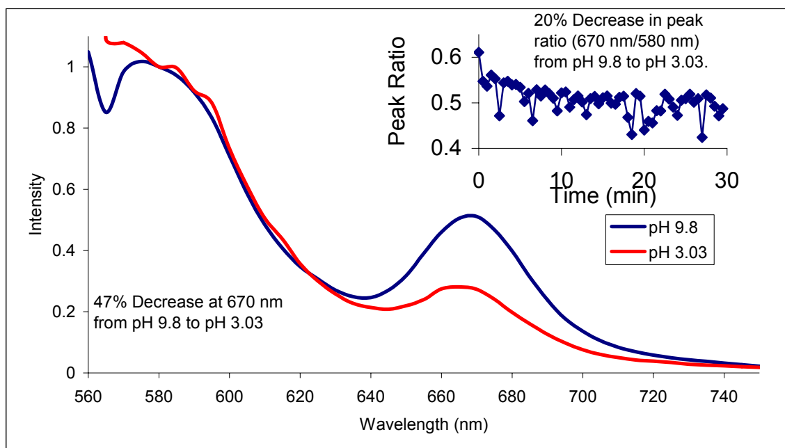
Figure 104. Transient pH response of microspheres (0.25% glutaraldehyde) from pH 9.8 to pH 3.03.
