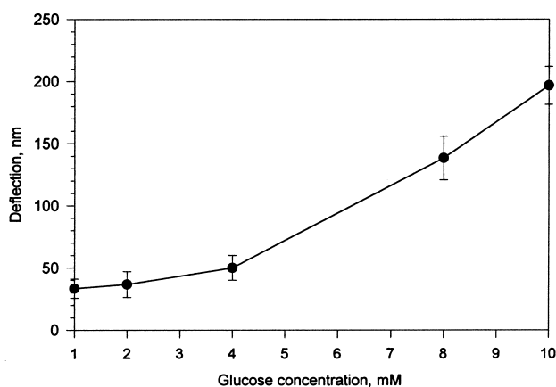
FIG. 2. Maximum bending amplitude for a microcantilever coated with a GOx-containing hydrogel as a function of the change in concentrations of glucose.
