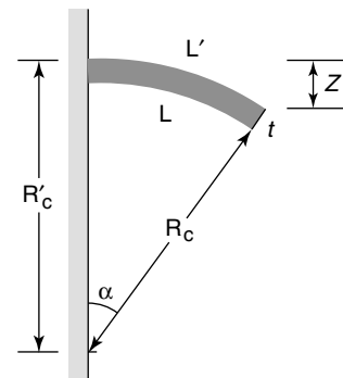
SCHEME A1. Schematic presentation of side and front views of a rectangular microcantilever.
