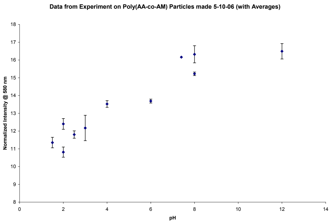
Figure 29: Ratio Value VS pH from pH Test on Poly(AA-co-AM) Microspheres Prepared with Emulsion Polymerization
