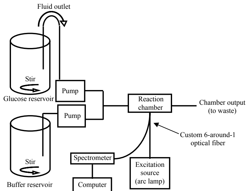
Figure 89. Schematic of dynamic testing apparatus used to quantify sensor response properties.
