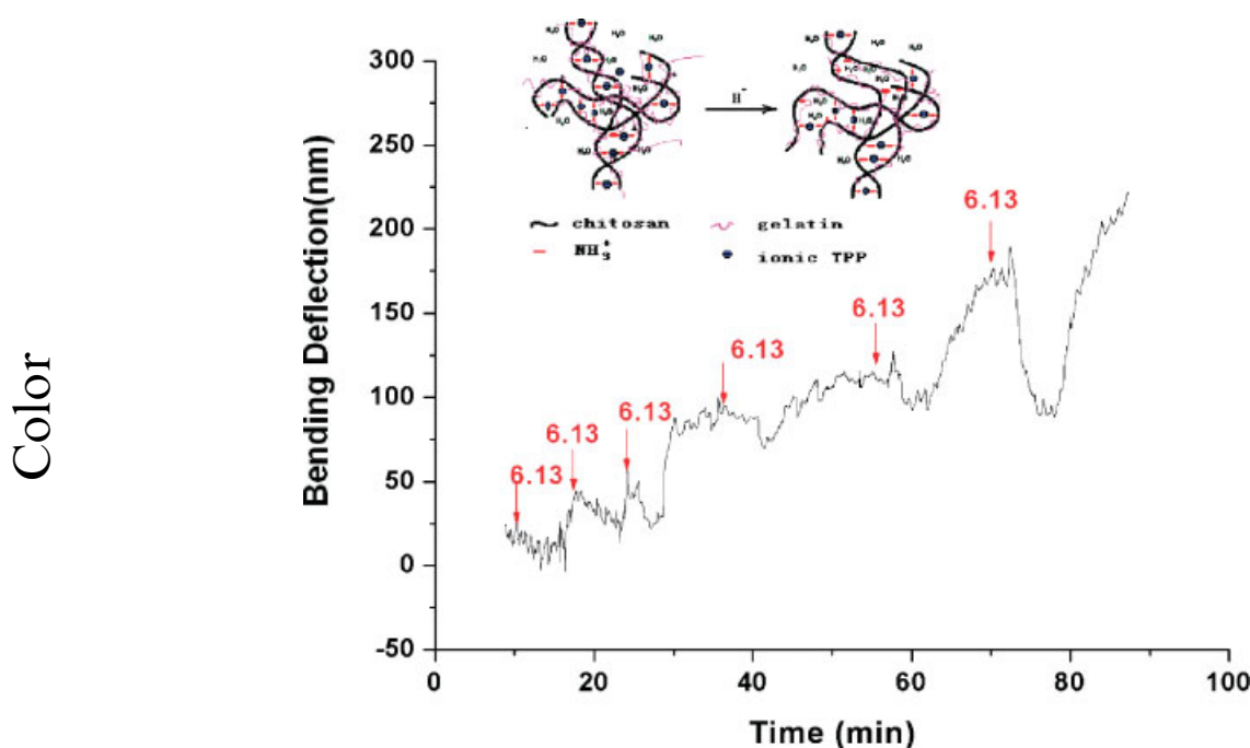
Figure 4. The transient bending response as a function of time for chitosan/gelatin (C:G = 1:1, 3.5% TPP at pH = 6.0) gel-coated microcantilever, upon injection of a 0.01M PBS at pH 6.13. Medium for baseline readings was 0.01M PBS, pH 7.45. Injection times are indicated with arrows.
