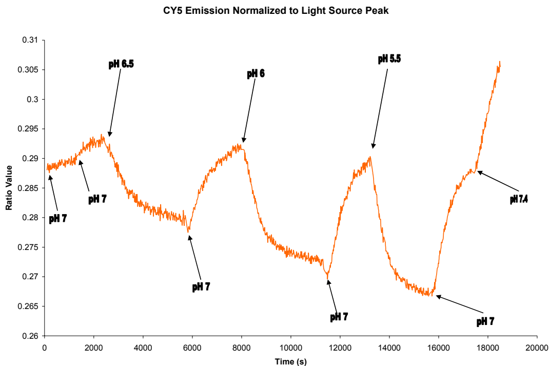
Figure 71: Response of CY5-Labeled Chitosan Hydrogel to Changes in pH
