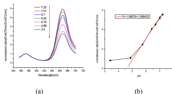
Figure 3: (a) FRET study in which TRITC and Alexa Fluor 647 TM dual labeled microspheres (b) Plot of the ratio of intensity (Em670nm/Em572nm) vs. the pH of the solution.
