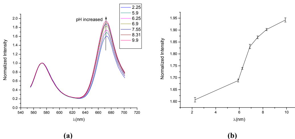
Figure 52: The fluorescent spectra of TRITC and Alexa Fluor 647 TM dual-labeled microspheres (Ex=543nm, Em=555-700nm) after normalized to TRITC peak at 572nm changed as the function of pH of 0.01M PBS solution. (a) The Alexa Fluor 647 TM /TRITC peak intensity ratio vs. pH (b) (Experiments were run in triplicate per sample. All data were expressed as means±standard deviation(SD) for n=3)
