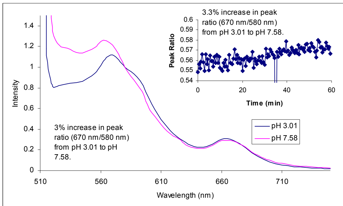
Figure 103. Transient pH response of microspheres (0.25% glutaraldehyde) from pH 3.01 to pH 7.58.
