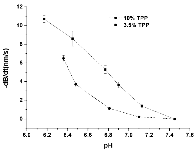
Figure 8. Maximum response speed ( -\text{dB}/\text{dt} ) as a function of pH for microcantilevers coated with chitosan/gelatin, crosslinked with different amounts of TPP at pH 6.0.
