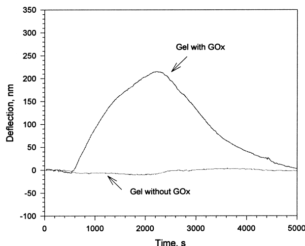
FIG. 3. Bending response as a function of time, t , for silicon microcantilevers coated with and without GOx-doped hydrogel on the gold surface after injection of a solution of 0.01 M glucose in 0.01 M NaCl. The microcantilevers were pre-equilibrated in the 0.01 M NaCl solution before injection of the glucose solution.
