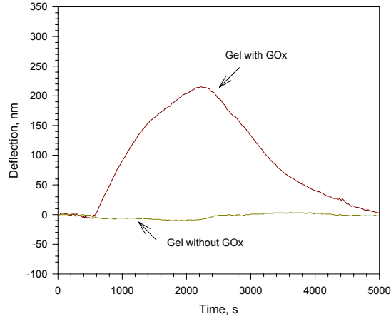
Figure 29: Bending response as a function of time, t , for silicon microcantilevers coated with and without GOx doped hydrogel on the gold surface after injection of a solution of 0.01M glucose in 0.01M NaCl. The microcantilevers were pre-equilibrated in the 0.01M NaCl solution before injection of the glucose solution.
