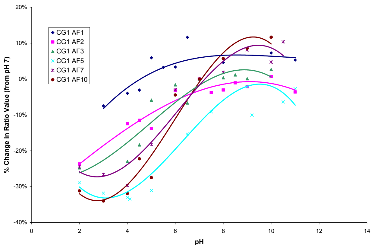
Figure 67. Change in fluorescence intensity ratio of chitosan microspheres at different pH. The different symbols and colors indicate varying labeling ratios.
