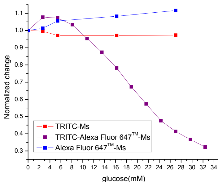
Figure 62: The normalized change of TRITC, or Alexa Fluor 647™ labeled microspheres, and TRITC and Alexa Fluor 647™ dual-labeled chitosan microspheres with loaded GOx response to glucose concentration. (Experiments were run in triplicate per sample. All data were expressed as means±standard deviation (SD) for n=3)
