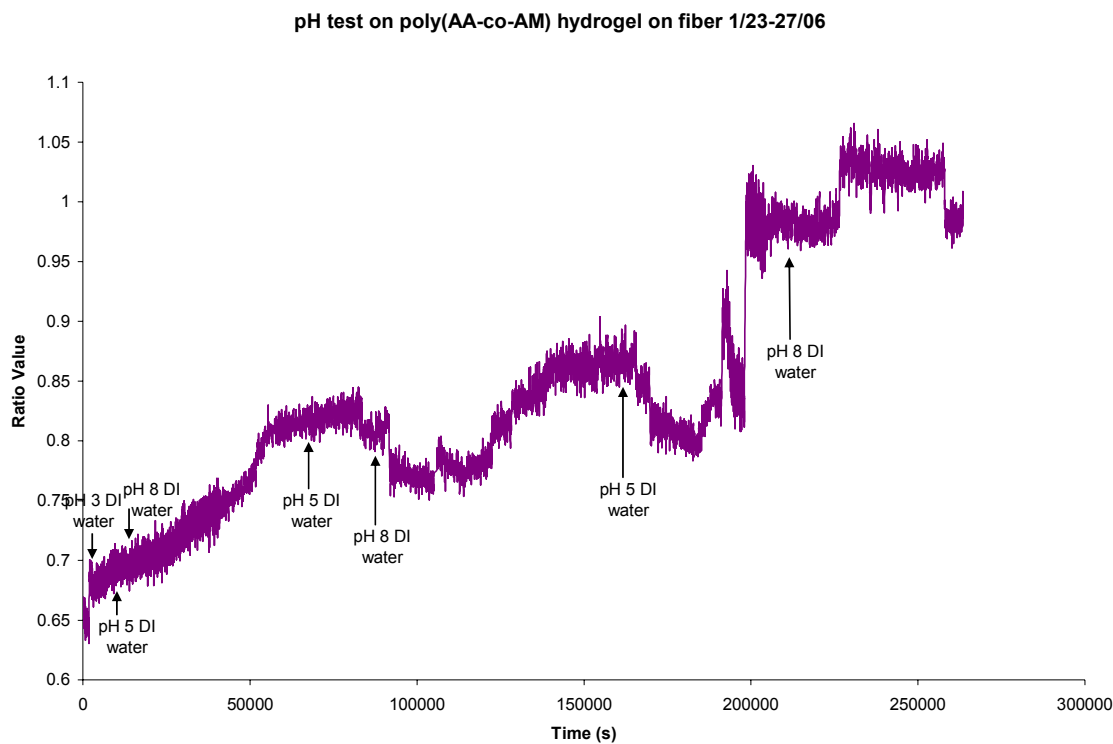
Figure 79: Best Results from pH Testing on Poly(AA-co-AM) Hydrogels on Optical Fiber
