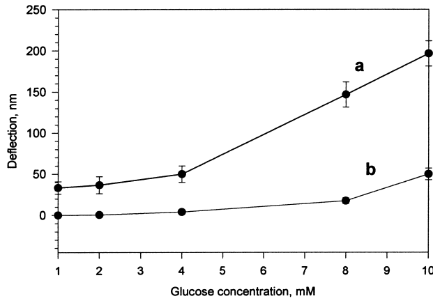
FIG. 5. Maximum bending amplitude for a microcantilever coated with a GOx-containing hydrogel as a function of the change in concentrations of glucose after equilibration for 1 day (curve a) and 30 days (curve b) in a 0.01 M NaCl solution.
