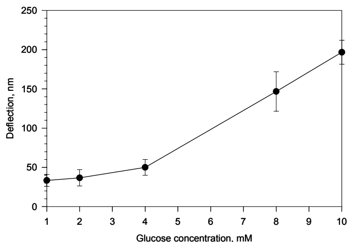
Figure 28: Maximum bending amplitude for a microcantilever coated with a GOx-containing hydrogel as a function of the change in concentrations of glucose
