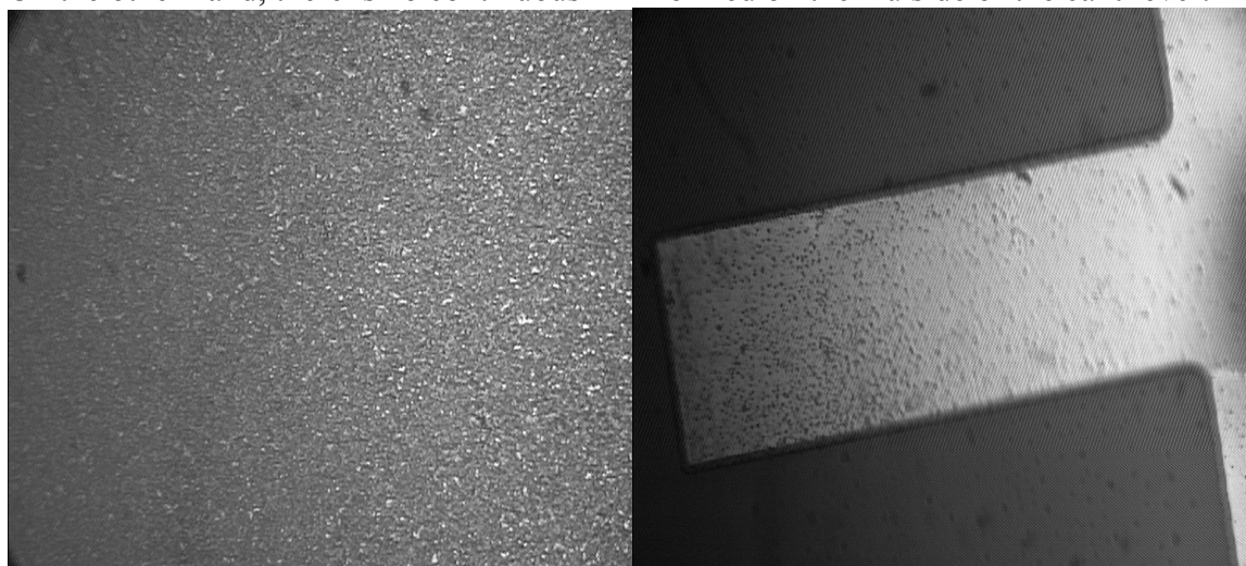
Figure 35. Au surface of wafer (Left) and the Au surface of the cantilever (Right) after the hydrogel microsphere LbL absorption. (Magnification \times 750).
