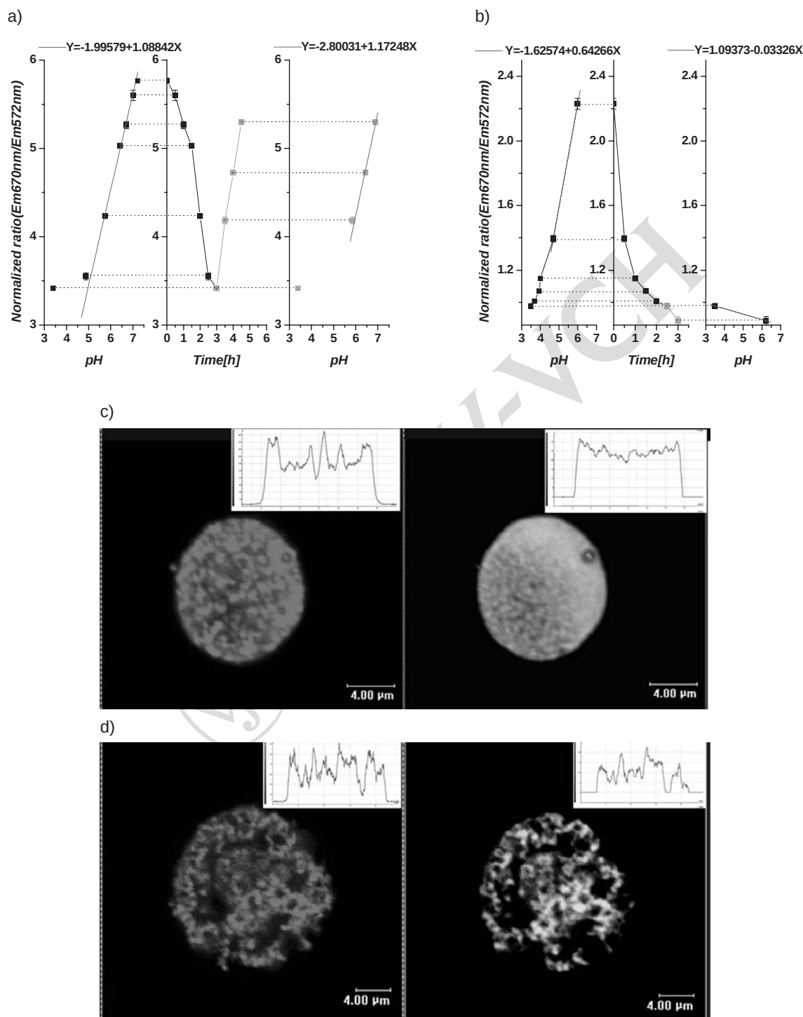
Figure 3. Fluorescence intensity ratios collected from microspheres during pH sensitivity tests a) with and b) without light glutaraldehyde crosslinking; confocal laser scanning microscopy images and internal dye distribution of dual-labeled microspheres c) with and d) without glutaraldehyde after repeated pH-response tests. The images have left (red) and right (yellow) panels corresponding to TRITC and AF 647 emission channels, respectively. The insets are intensity line scans across each particle, indicating the distribution of fluorescence inside the microspheres.
