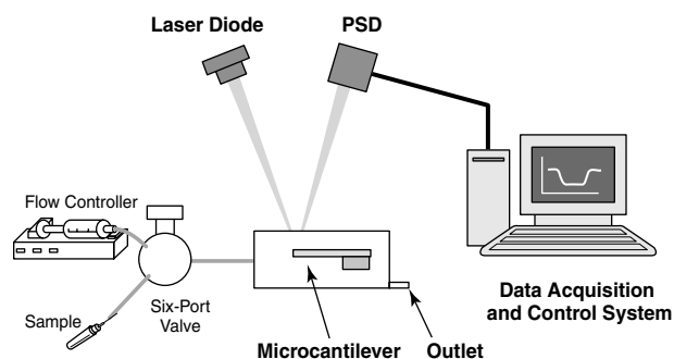
SCHEME 1. Schematic diagram of the deflection measurement apparatus used in this study. PSD, position-sensitive detector.
