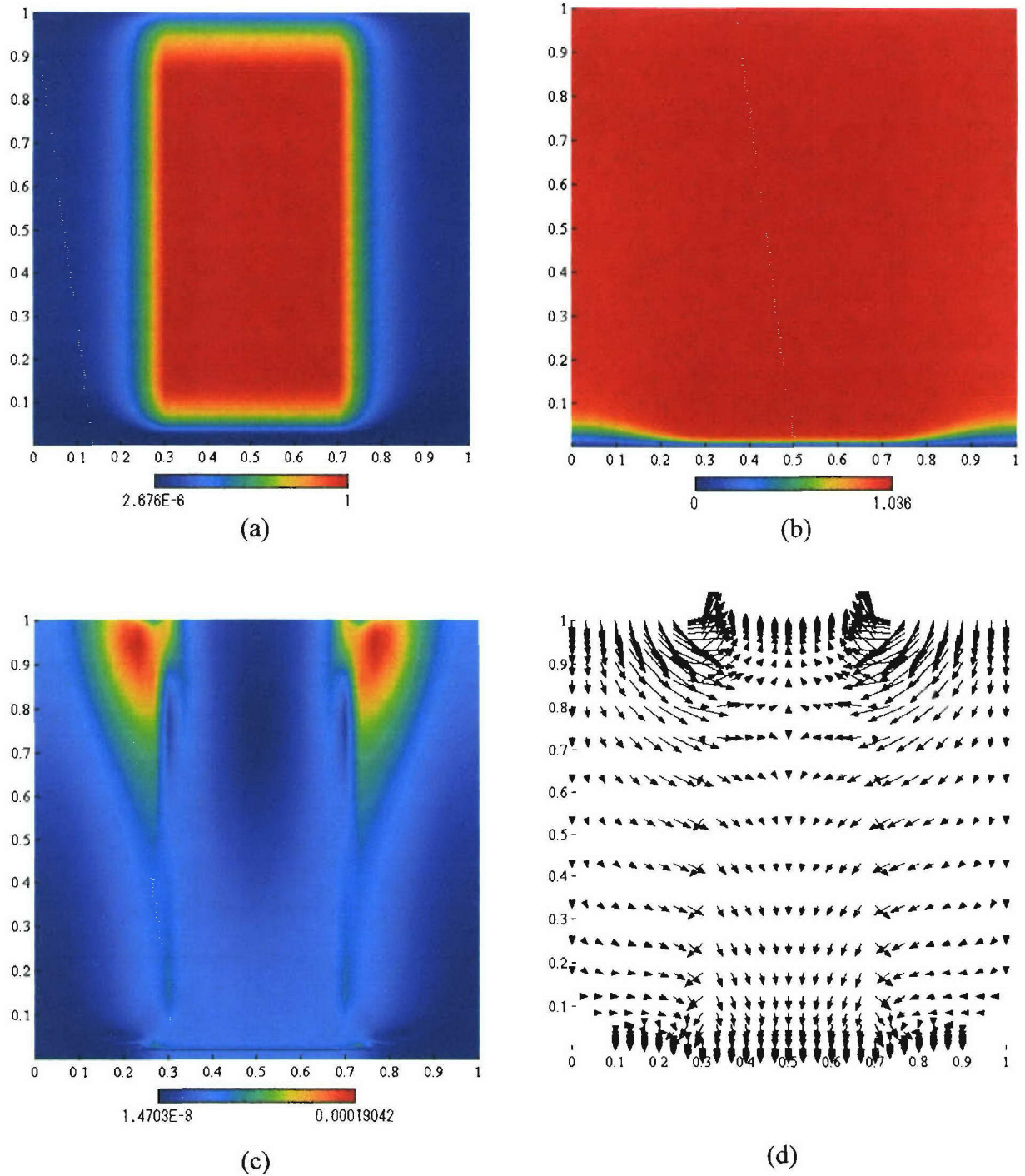
Figure 23. Electron density distribution (a), potential distribution (b), current distribution (c), and current vector field (d) in a non-self-sustained DC discharge with no B field applied. U=50 V, maximum electron density n_e=2 \cdot 10^{11} cm 3 /sec (electrical conductivity of 0.074 mho/m), secondary emission coefficient \gamma=1.0 . Discharge current is 0.52 mA.
