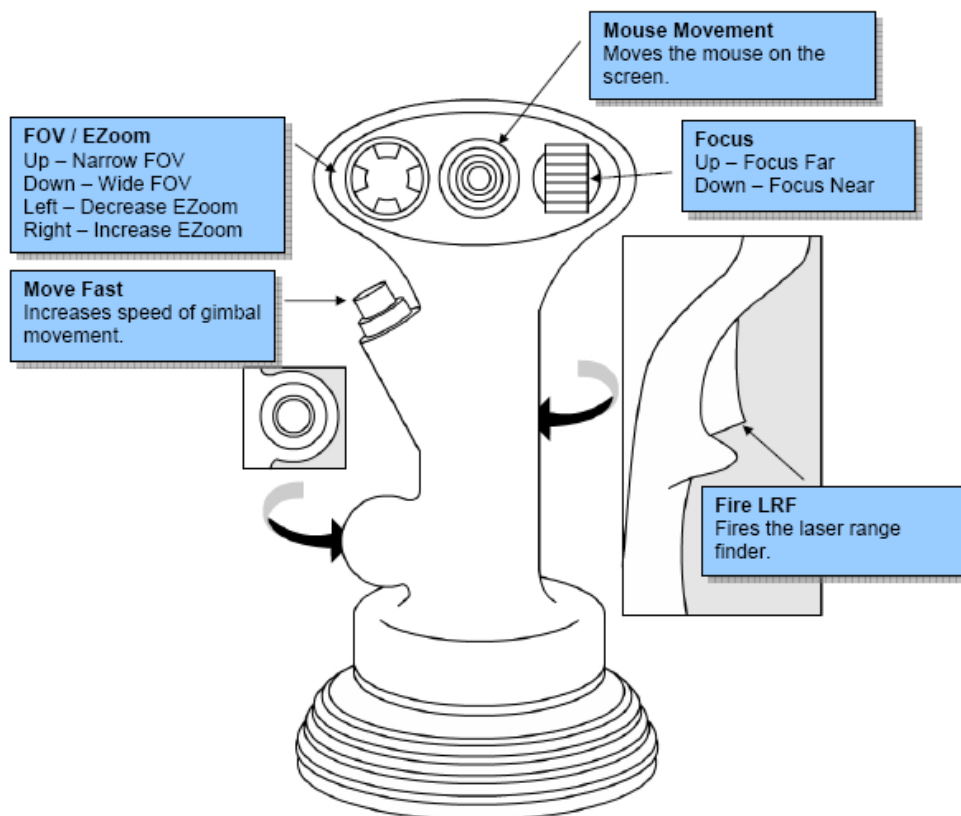
Joystick Control
