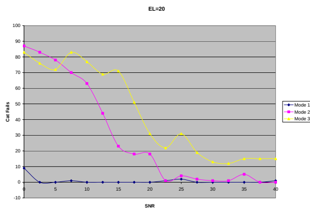
Figure 16: SNR vs. # of catastrophic failures for \theta = 20^\circ at 4GHz.
