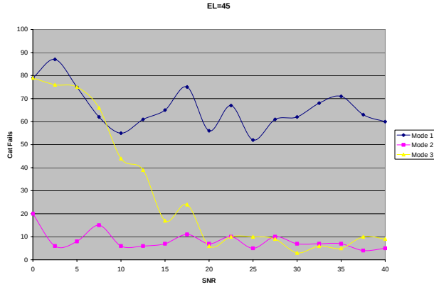
Figure 18: SNR vs. # of catastrophic failures for \theta = 45^\circ at 4GHz.
