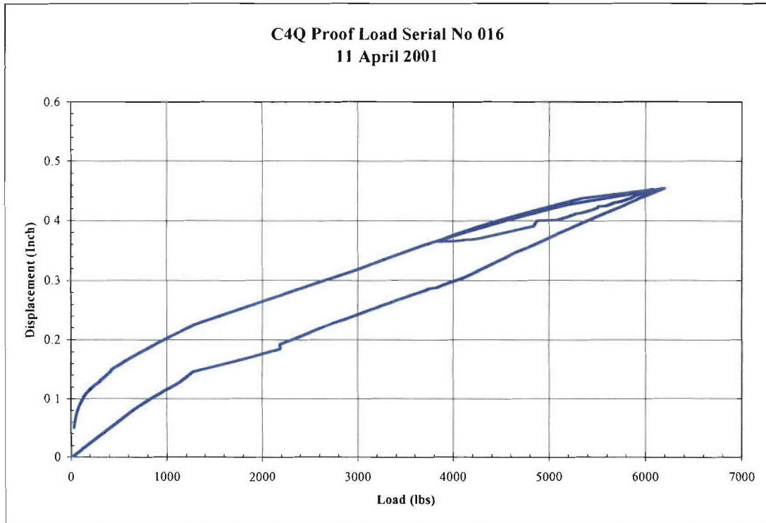
FIGURE W-9. Load Versus Displacement for Blue Tube Serial Number 016.
