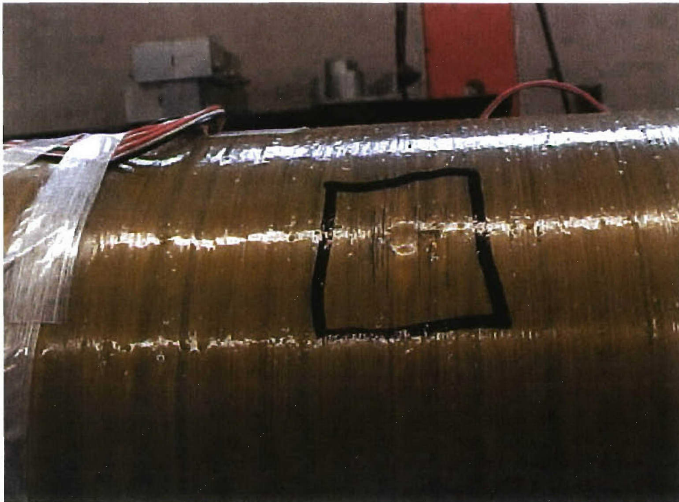
FIGURE D-5. Aft Impact Damage Location.
