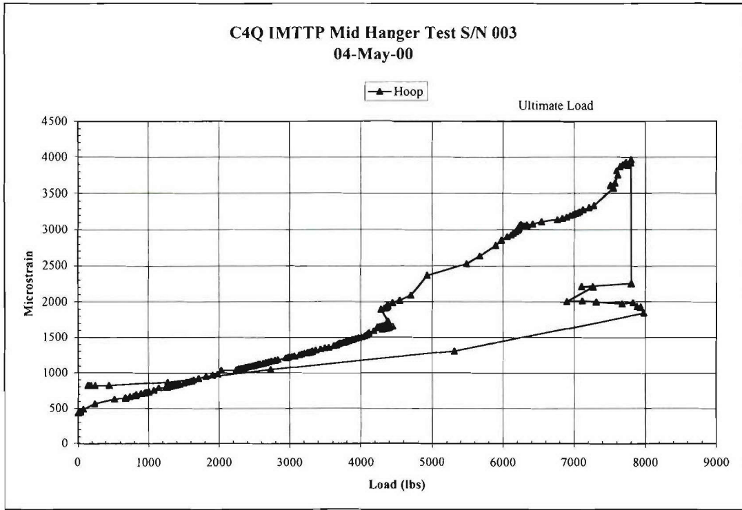
FIGURE H-7. Ultimate Test Hoop Strain Data (No Release).
