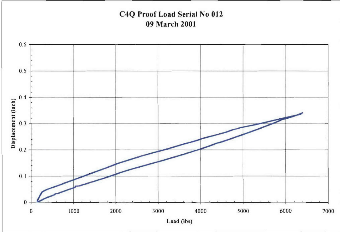
FIGURE W-5. Load Versus Displacement for Blue Tube Serial Number 012.
