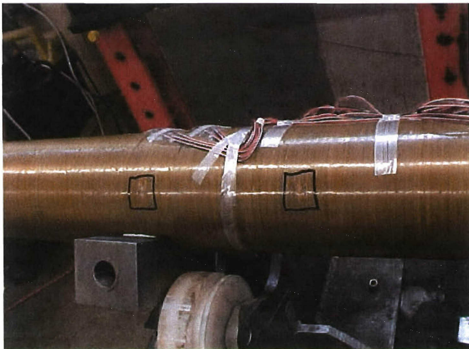
FIGURE D-3. Impact Damage Locations.
