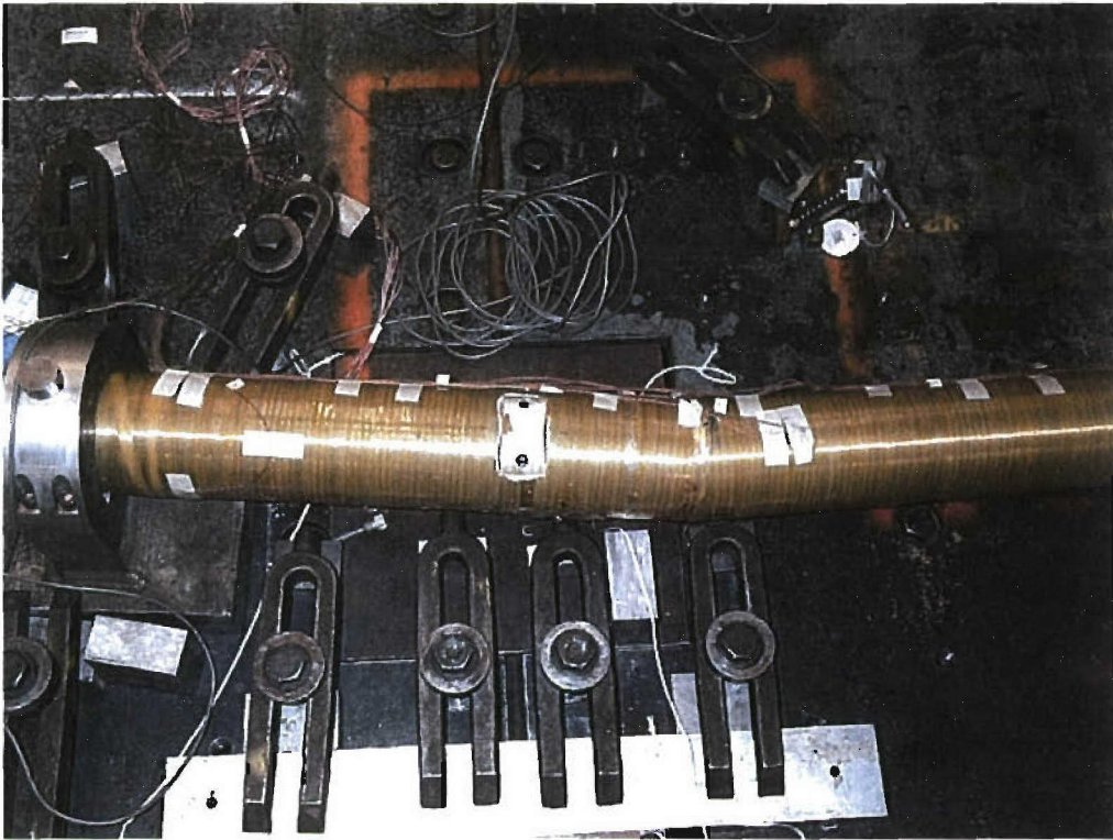
FIGURE D-14. Failure Photograph 1.
