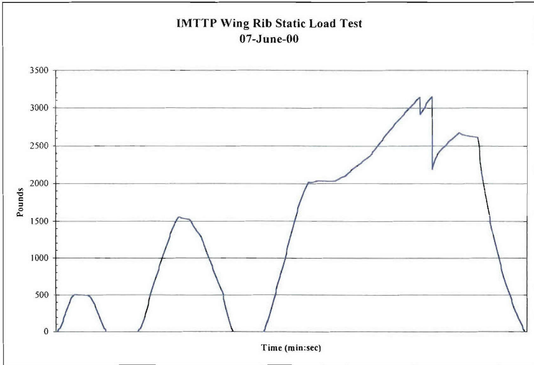
FIGURE N-4. Wing Attachment Test Load History.
