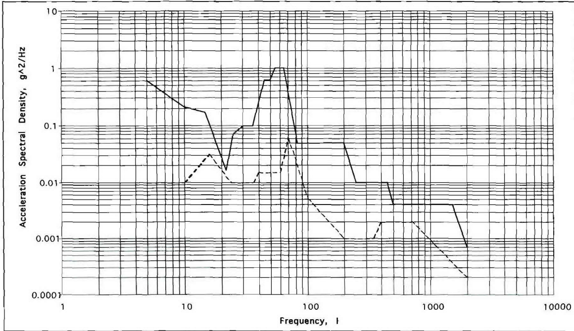
Vertical and Transverse (Solid Line) Longitudinal (Dashed Line) 0 dB, 5 min/axis -2.5 dB, 38 min/axis -6.0 dB, 128 min/axis
