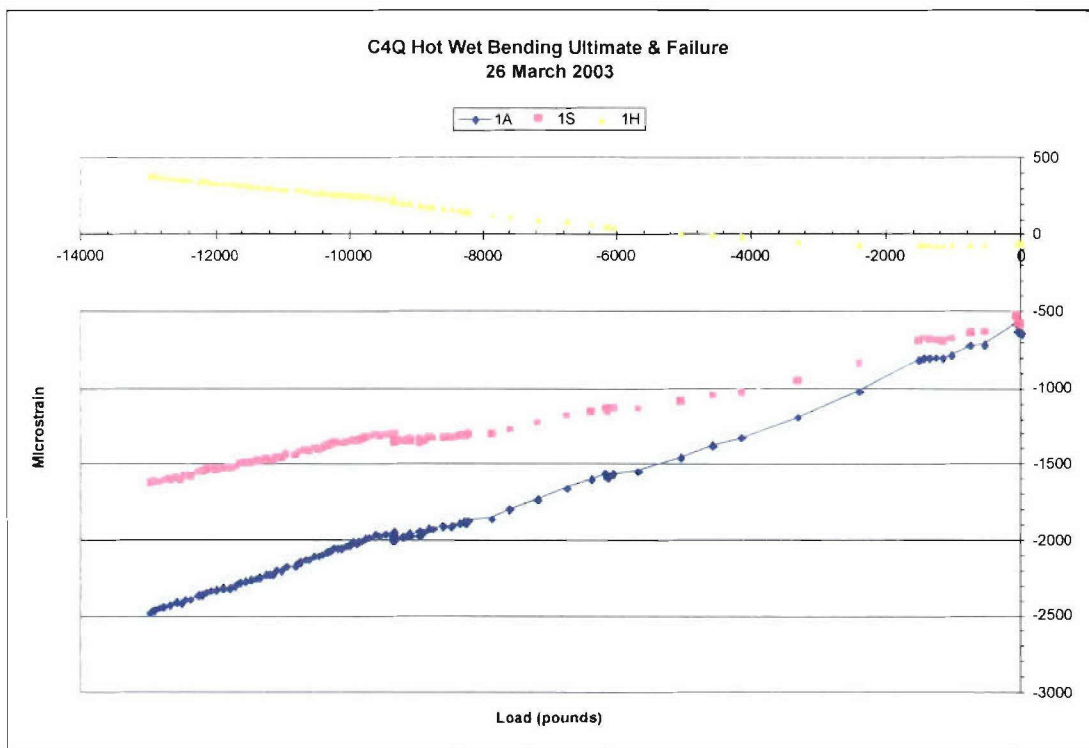
FIGURE X-13. Strain Gage 1 Ultimate and Failure Load.
