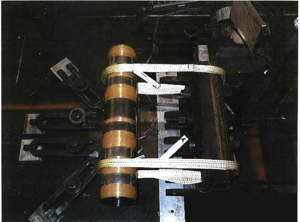
FIGURE L-2. Aft Hanger Loading Fixture.
