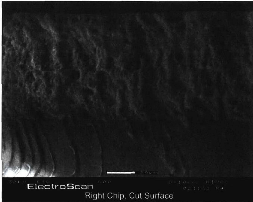
FIGURE Y-12. SEM Micrograph Showing Cut Surface of Right Chip (600X Magnification).
