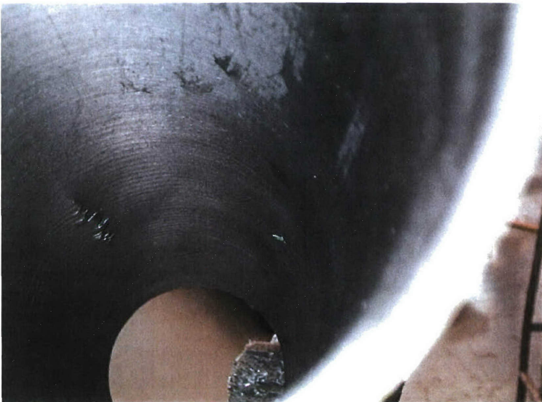
FIGURE H-9. Middle Hanger Failure (No Release), Inside View.
