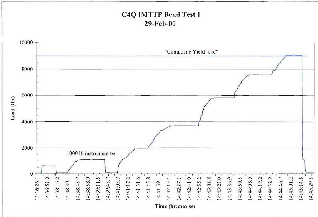
FIGURE B-5. Yield Test Load History.
