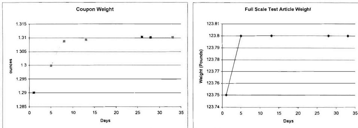
FIGURE D-6. Test Article and Coupon Weight Gain.
