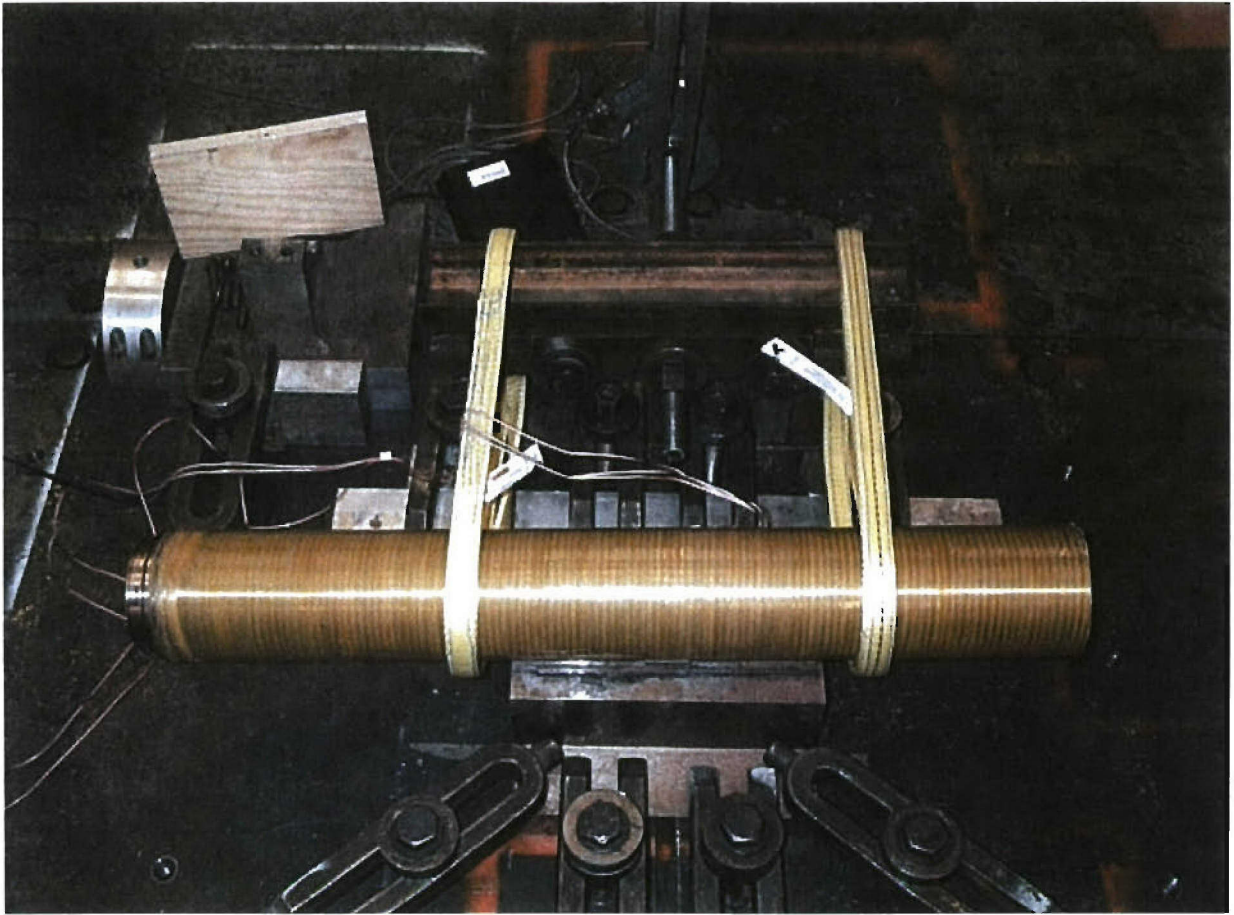
FIGURE F-2. Forward Hanger Loading Fixture.
