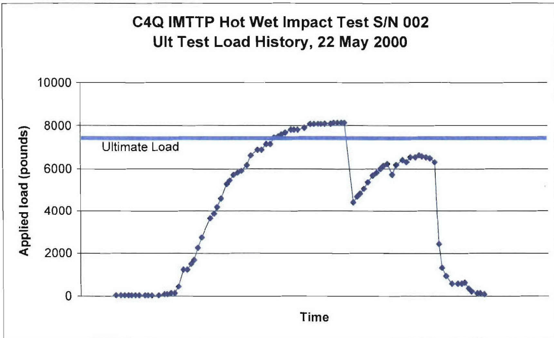
FIGURE D-11. Ultimate Test Load History.
