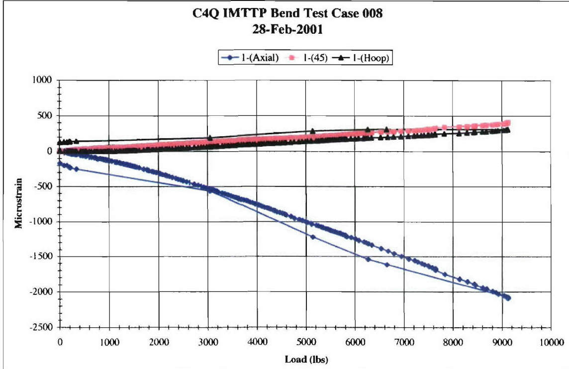
FIGURE T-22. Yield Condition Load vs. Microstrain, Gage 1 (Blue Tube Serial Number 008).
