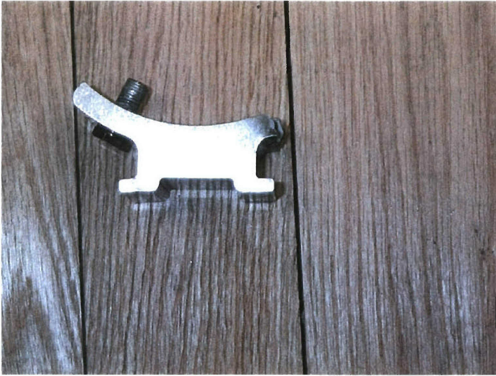
FIGURE F-7. Ultimate Load Test Hanger Failure Mode (Close-up).
