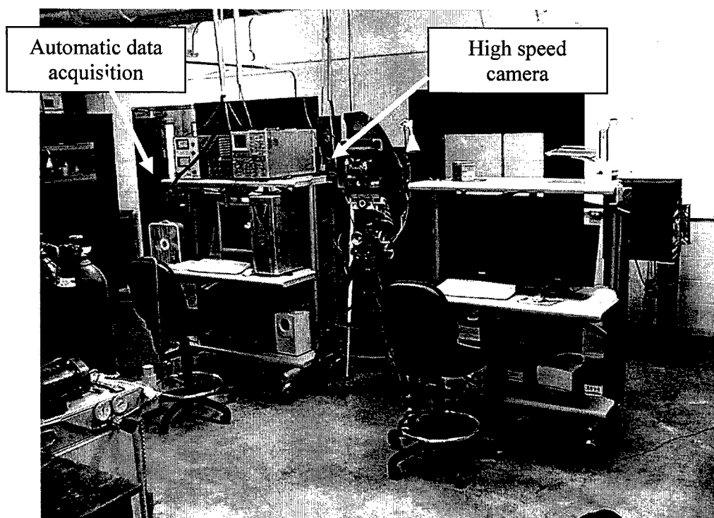
Fig 2. Computerized data acquisition system and high-speed camera.
