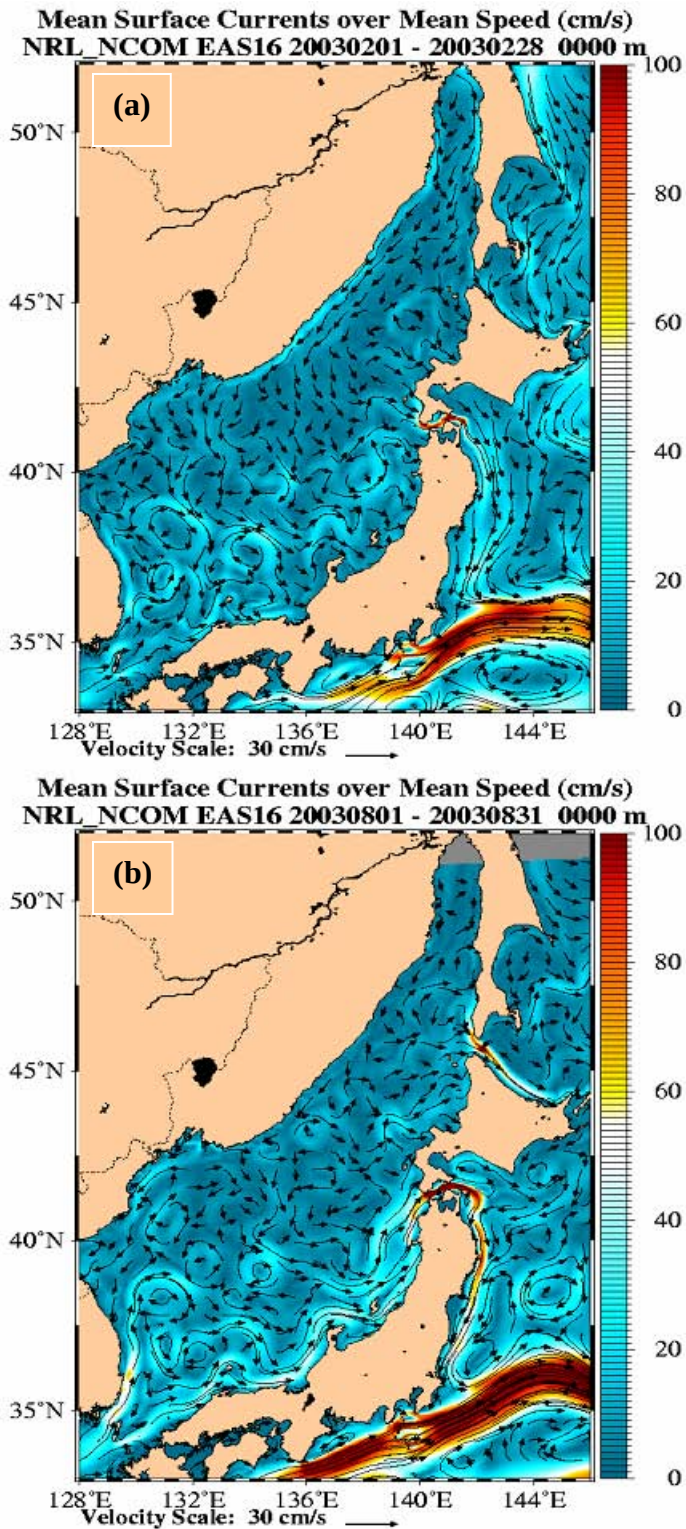
Figure 9 a-b. Monthly mean surface currents from EAS16 model for the Sea of Japan, a) February 2003, b) August 2003.
