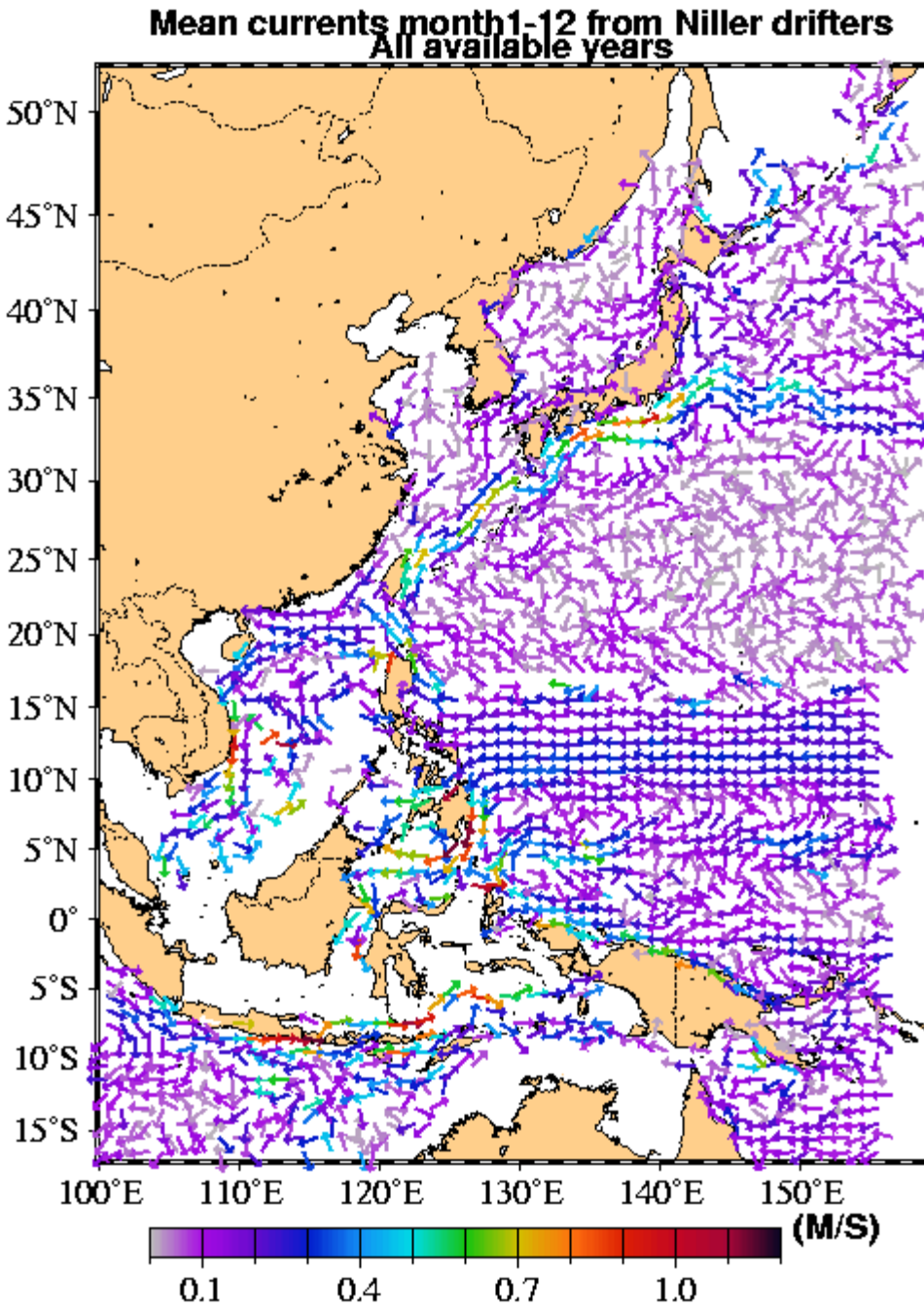
Figure 25a. Mean currents computed from Niiler drifter data in 1^\circ \times 1^\circ bins (all years and all months.) Empty bins occur as there are no drifter measurements in those areas. Color scale is speed in m/sec.
