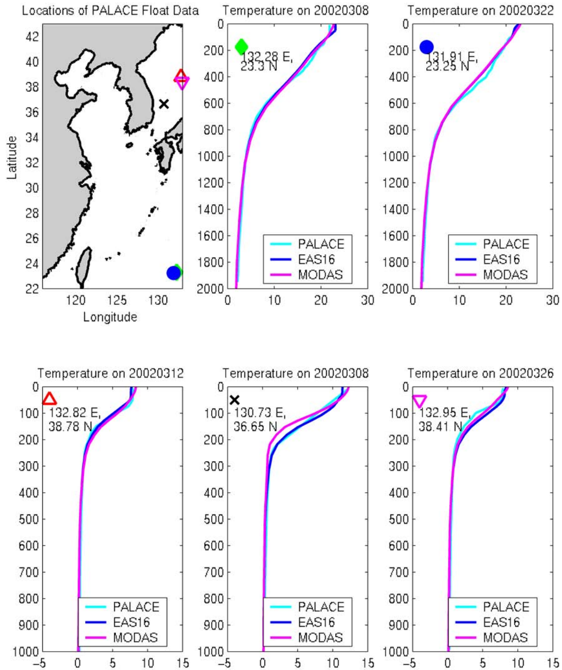
Figure 14. Comparison of temperature profiles from model (dark blue line), PALACE floats (cyan line), and MODAS (pink line) at locations in the Sea of Japan and Pacific south of Ryukyu Islands. (Plots provided by Andrea Mask.)
