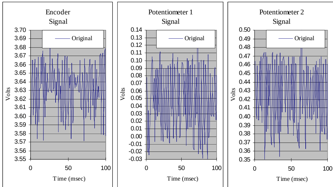
Figure 14. Measurements of voltage entering the data acquisition board when the mechanical linkage hung freely (original wiring).
