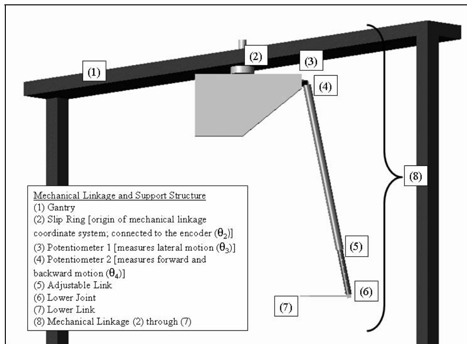
Figure 13. Mechanical linkage and support structure.
