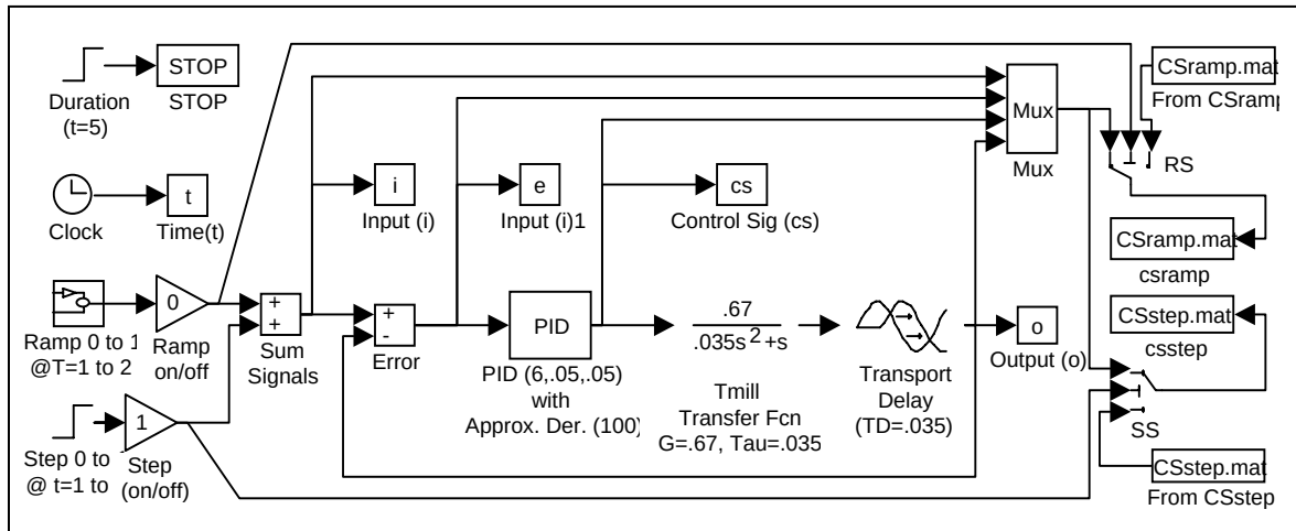
Figure 23. Final system model.
