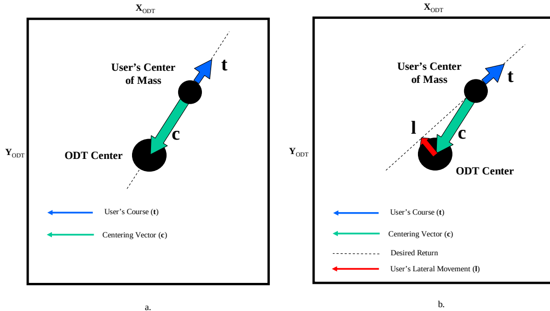
Figure 12. Course and centering vector (a) aligned and (b) misaligned.
