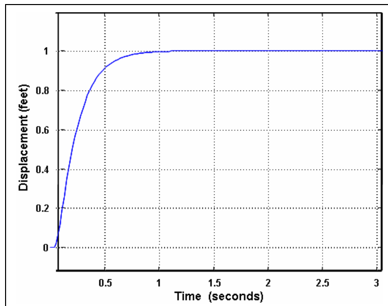
Figure 24. Response of the ODT system model to a unit voltage step input.
