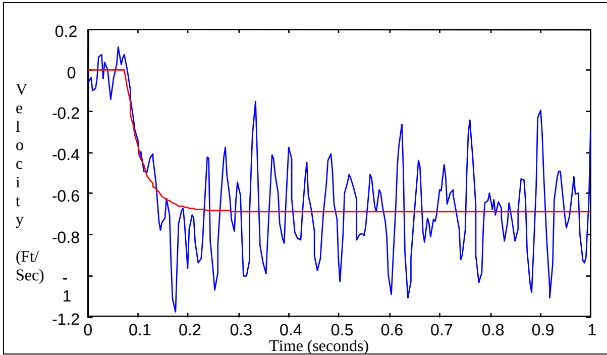
Figure 21. Velocity response of the inner belt to a unit voltage step input.
