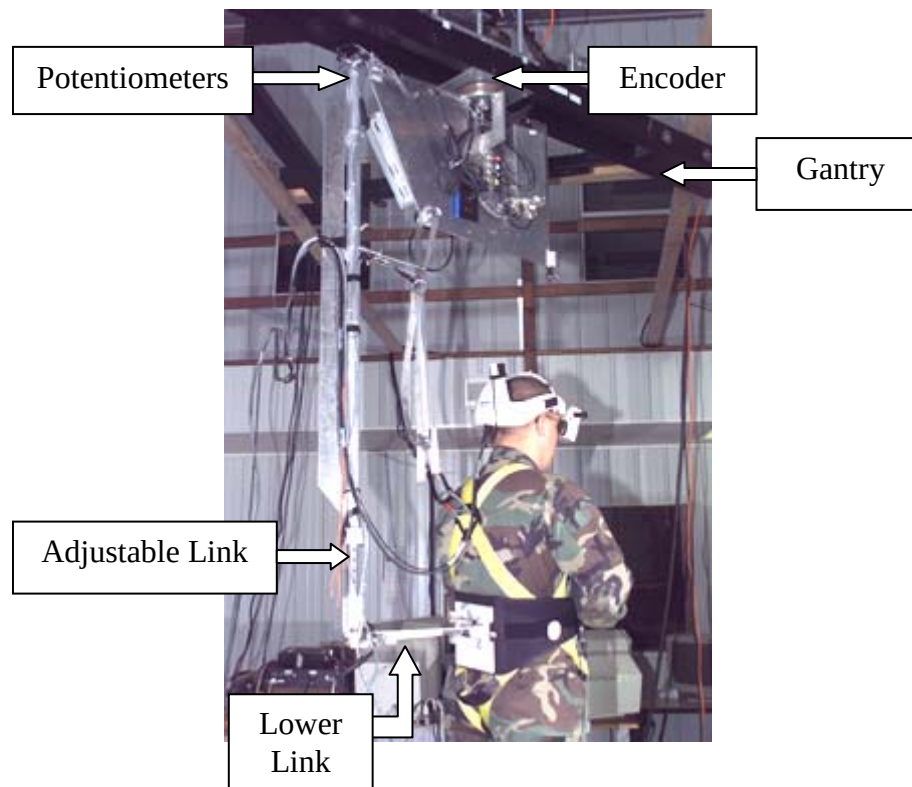
Figure 11. The mechanical linkage.
