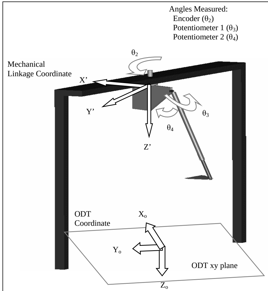
Figure 19. Coordinate systems and angles measured.
