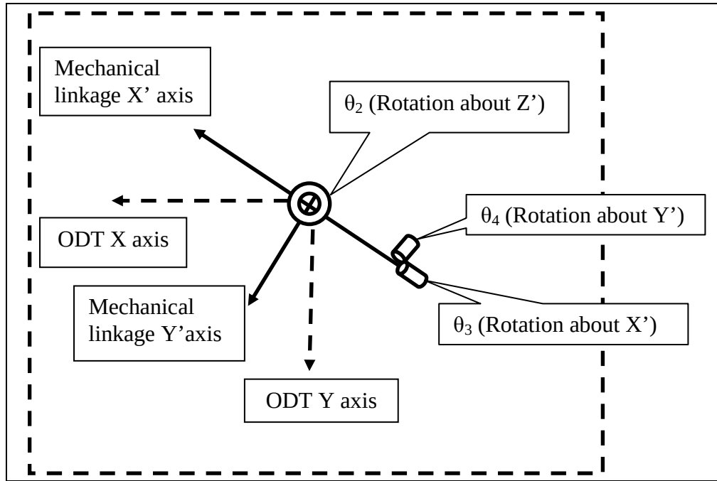
Figure 26. Top-down view of the mechanical linkage coordinate system ( X' , Y' , Z' ) and the ODT coordinate system ( X , Y , Z ). (The Z' and Z axes point downward.)
