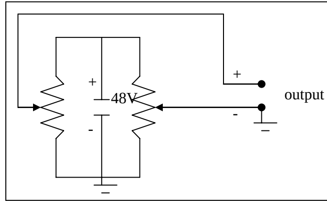
Figure 15. Potentiometer circuit.
