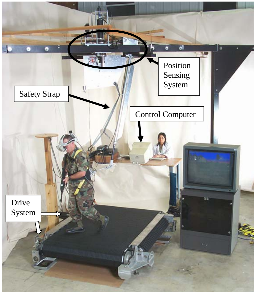
Figure 9. The ODT and its subsystems.
