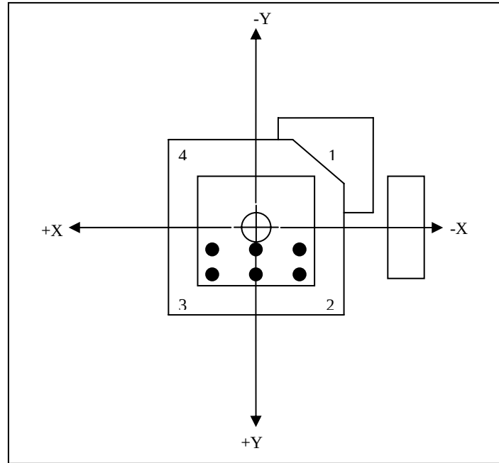
Figure 29. Locations of belt noise measurements.
