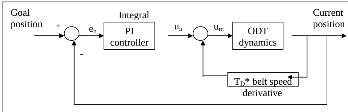
Figure 27. Block diagram of the ODT control.
