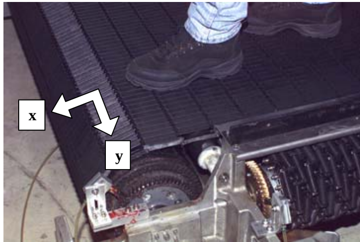
Figure 10. The rollers that comprise the active surface of the ODT.
