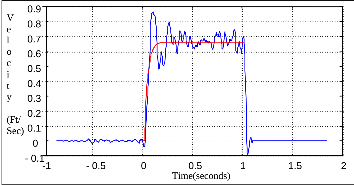
Figure 20. Velocity response of the outer belt to a unit voltage step input.
