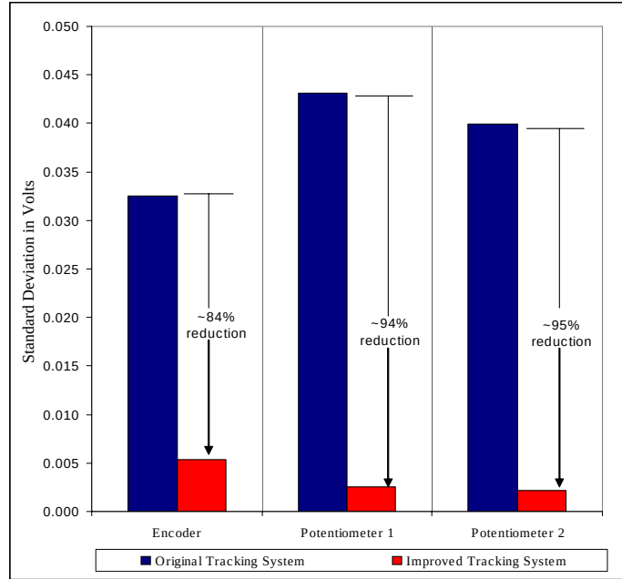
Figure 17. Comparison of standard deviations in the voltages after the improvements in the wiring.
