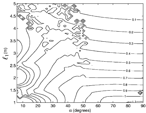
Fig. 14. Contours of relative bandgap \frac{\omega_2 - \omega_1}{\sqrt{|\omega_1 \omega_2|}} for l_1 versus \alpha angle.
