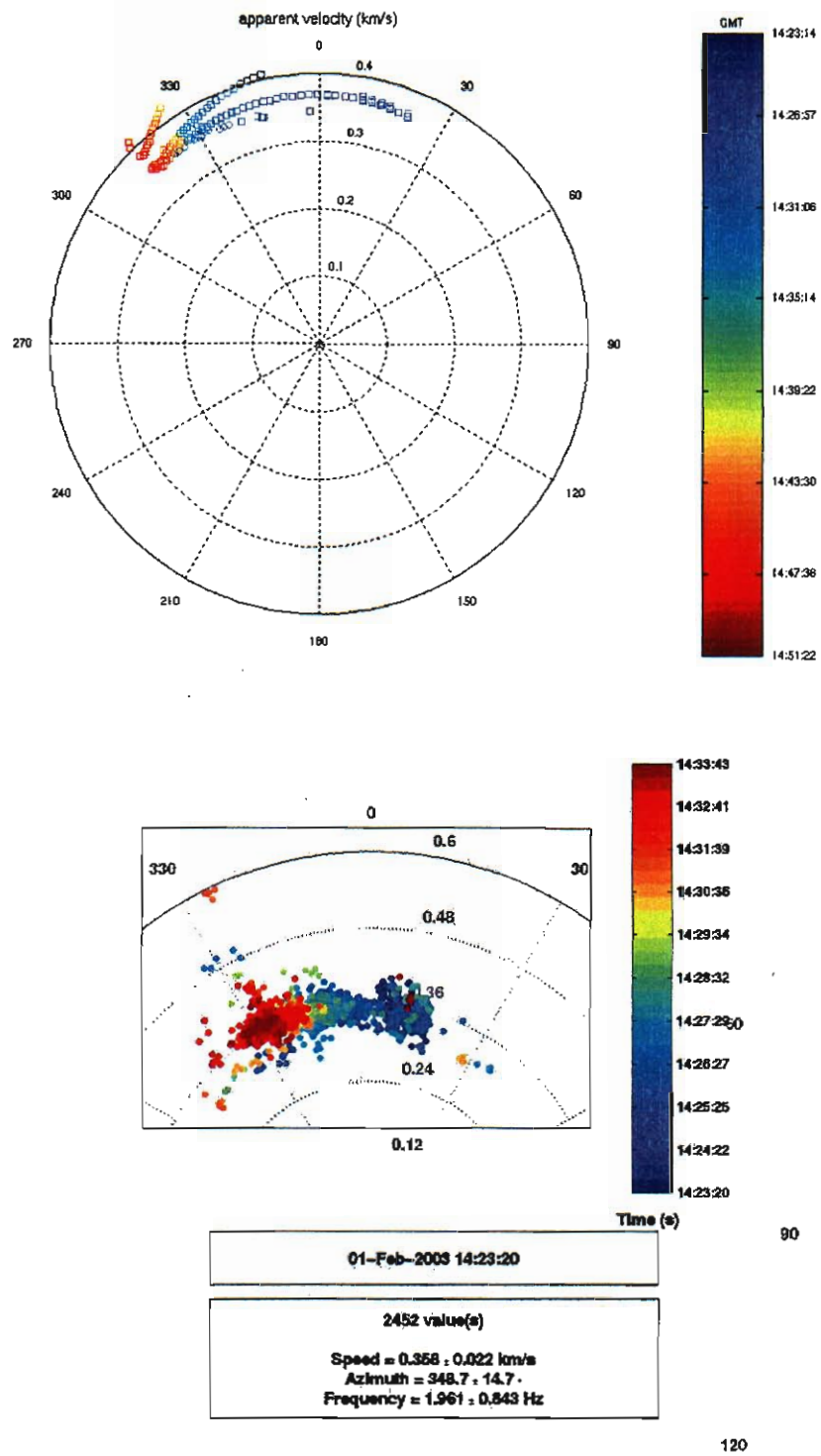
Figure 2. HARPA predictions (upper panel, Gibson and Norris, 2003b) and PMCC observations (lower panel) for I57US.
