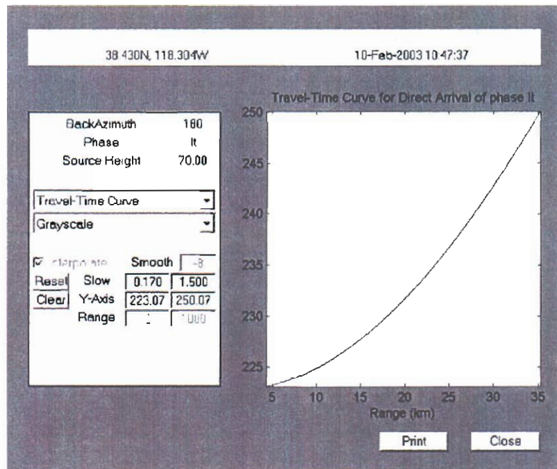
Figure 5. Travel time for the direct arrival at NVIAR for a source south of the array at a height of 70 km.
