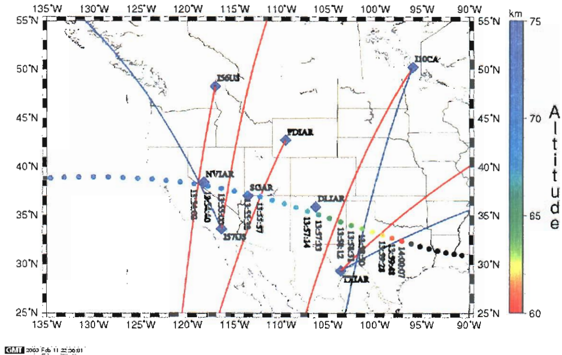
Figure 17. Projected track, altitude, time GMT, and infrasonic detections for the Columbia reentry.
