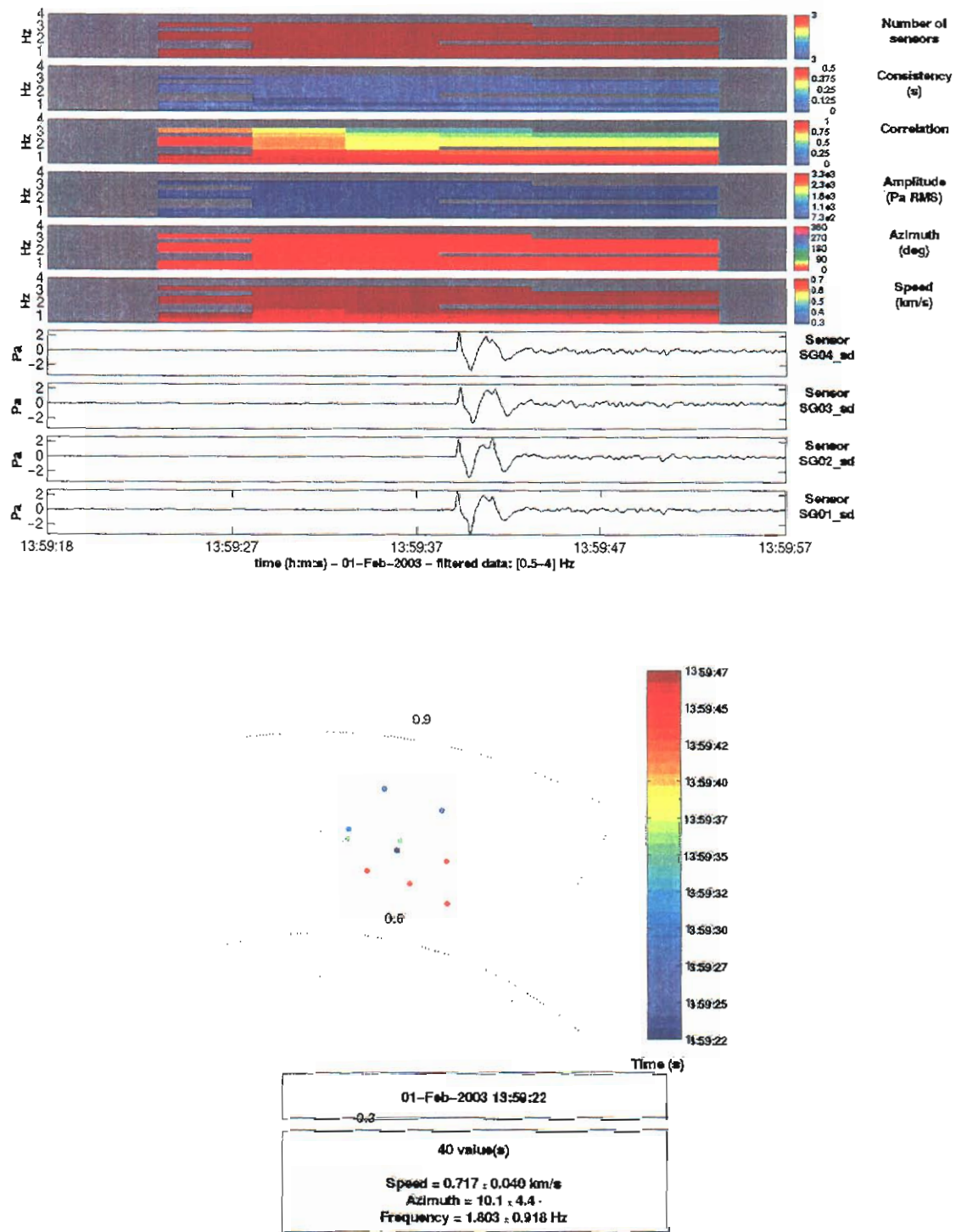
Figure 8. Possible bow wave observed in the 0.5- 4 Hz band at SGAR and associated with the Columbia reentry.
