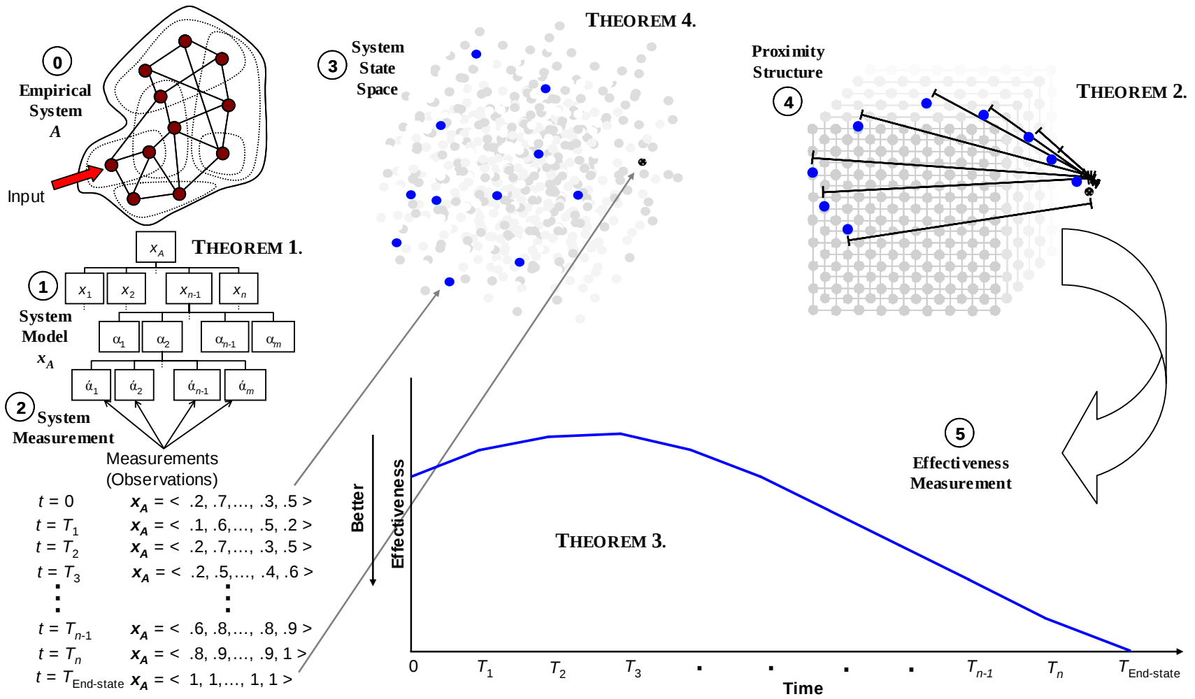
Figure 12. Framework Summary
