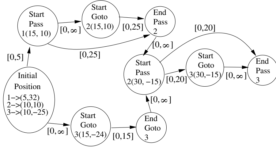
Figure 6.2: An example MASTN. The nodes represent events and the edges represent temporal constraints. The agent responsible for bringing about the occurrence of the event is shown inside each node. The numbers in parentheses are vectors representing locations on the field (elements of \mathcal{L} ). These vectors are the parameters to the various node types. The node pointers are not explicitly represented in this picture. This plan corresponds to the execution depicted in Figure 6.1.
