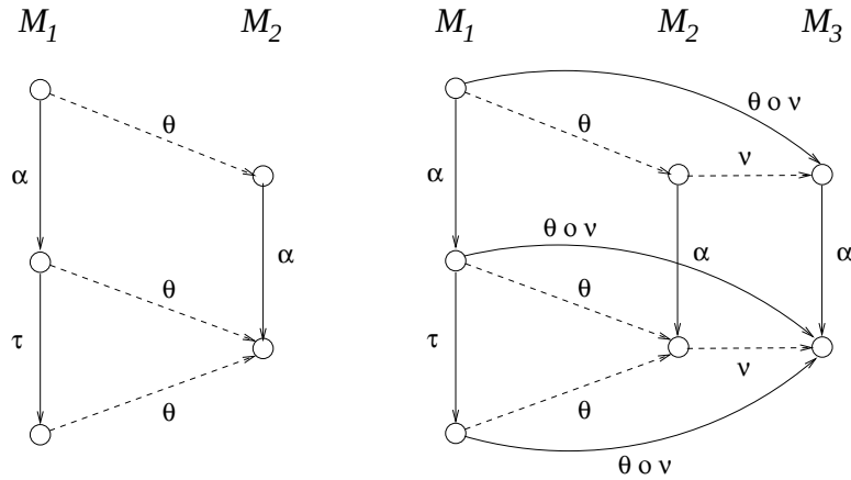
Figure 9.1: On the left is a simulation map \theta between M_1 and M_2 . On the right is a simulation map \theta \circ \nu between M_1 and M_3 .
