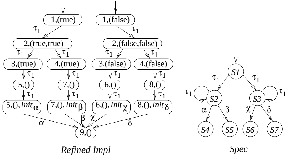
Figure 6.2: On the left is the refined abstraction of the component from Figure 6.1 using states \{3, 4\} as seeds. The empty valuation \perp is written as () . On the right is the specification from Figure 5.3. Note that the refined abstraction is simulated by the specification.
