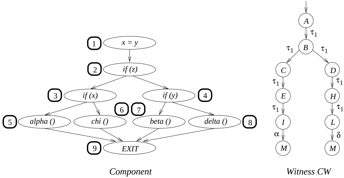
Figure 6.1: The component from Figure 4.1 and CounterexampleWitness from Figure 5.4. Note that the CounterexampleWitness is spurious.
