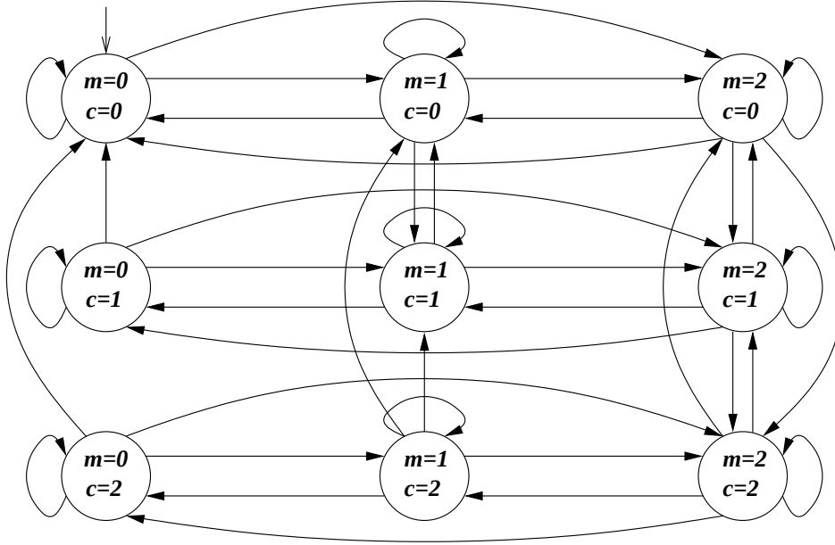
Figure 8.2: The Kripke structure of a surge protector
