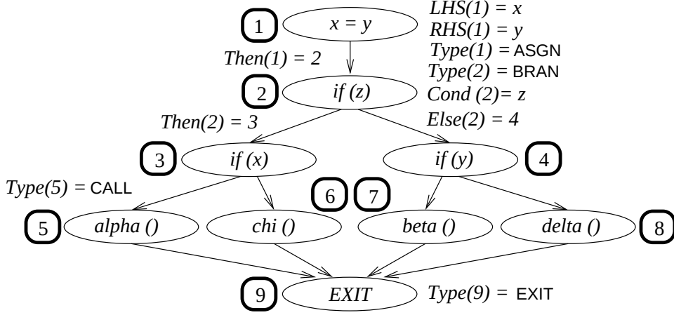
Figure 3.2: Component for the C procedure shown in Figure 3.1. We will use this as a running example.
