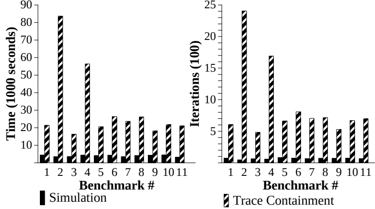
Figure 6.3: Comparison between simulation and trace containment in terms of time and number of iterations.
