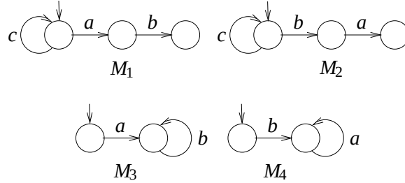
Figure 10.2: Four sample LKSs demonstrating the non-compositional nature of deadlock.
