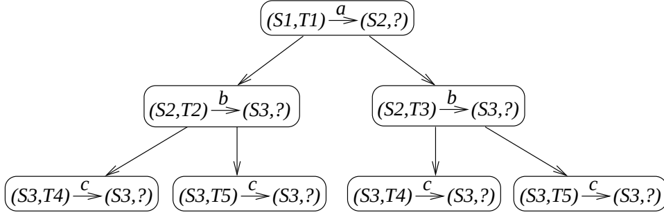
Figure 5.2: Counterexample Tree for a simulation game.
