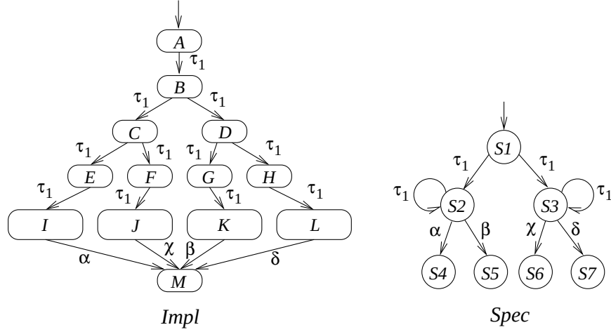
Figure 5.3: An implementation Im and a specification Sp . Im is the LKS from Figure 4.2.
