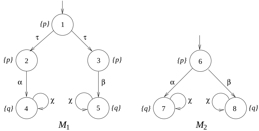
Figure 2.3: Two LKSs demonstrating weak simulation.
