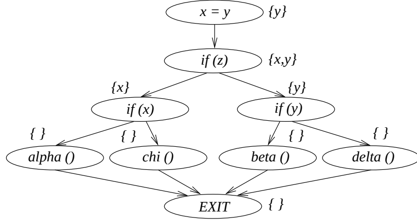
Figure 4.3: The component of Figure 4.1 with each statement labeled by inferred predicates computed by PredInfer from the set of seed branches \{3, 4\} .
