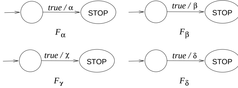
Figure 3.4: The EFSMs corresponding to the context from Example 9.
