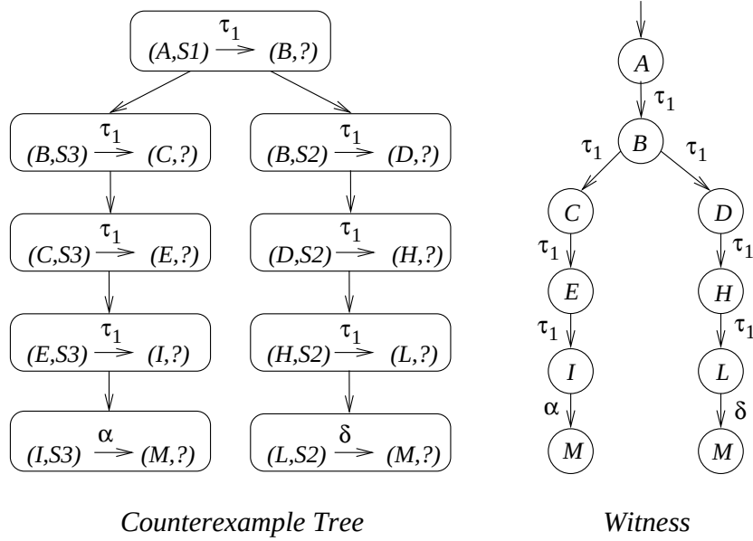
Figure 5.4: A CounterexampleTree and CounterexampleWitness corresponding to the simulation game between Im and Sp from Figure 5.3. Each state of the CounterexampleWitness is labeled by the corresponding state of Im which simulates it.
