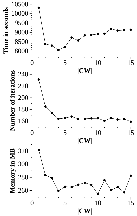
Figure 6.4: Time, iteration and memory requirements for different number of Counterexample Trees.
