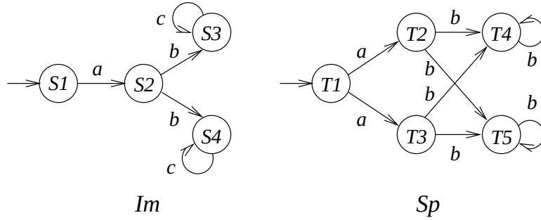
Figure 5.1: Two simple LKSs.
