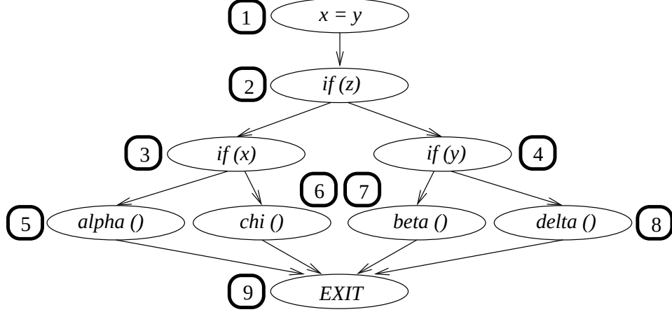
Figure 4.1: The component from Example 9.
