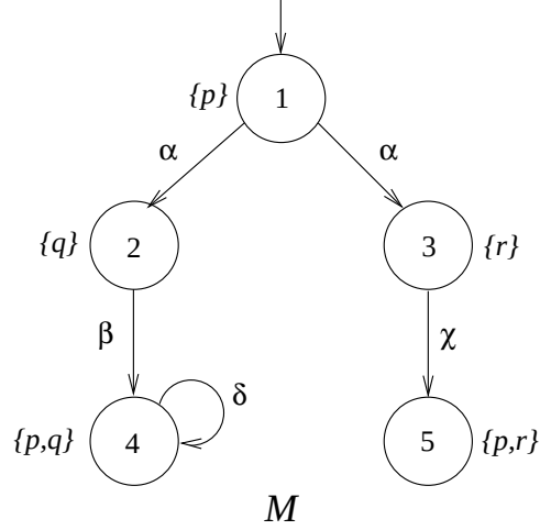
Figure 2.1: A simple LKS.
