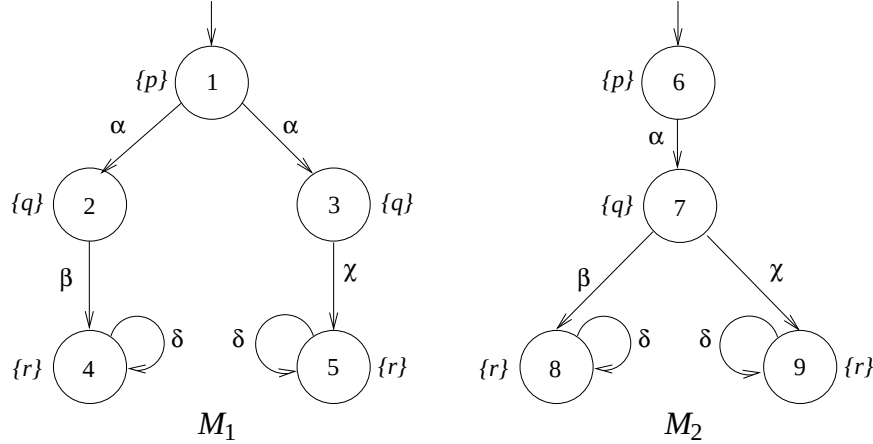
Figure 2.2: Two LKSs demonstrating simulation.
