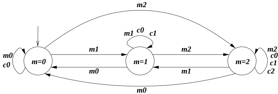
Figure 8.1: The LKS of a surge protector
