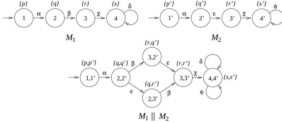
Figure 2.5: Three LKSs demonstrating parallel composition.
