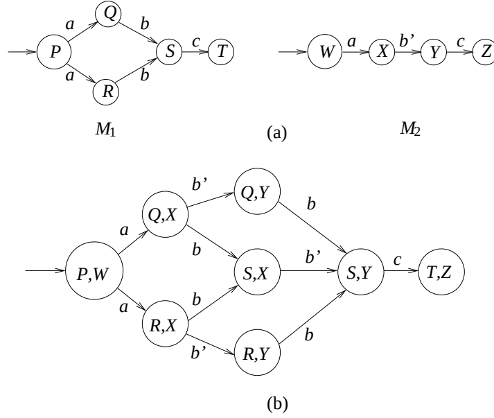
Figure 10.1: (a) Sample LKSs M_1 and M_2 ; (b) M_1 \parallel M_2 .
