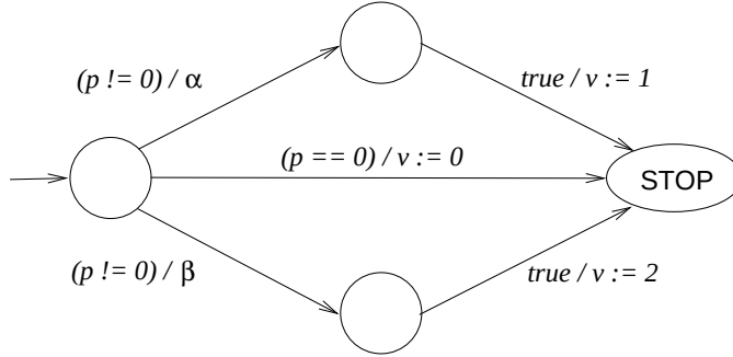
Figure 3.3: The EFSM corresponding to the library routine from Example 8. The initial state is indicated by an incoming transition with no source state.
