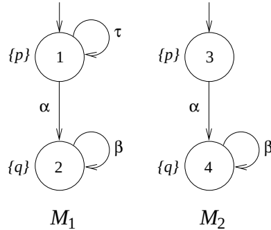
Figure 2.4: Two LKSs showing that weak simulation does not preserve liveness properties.
