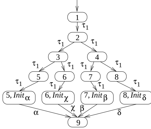
Figure 4.2: The LKS obtained by predicate abstraction of the component in Figure 4.1.
