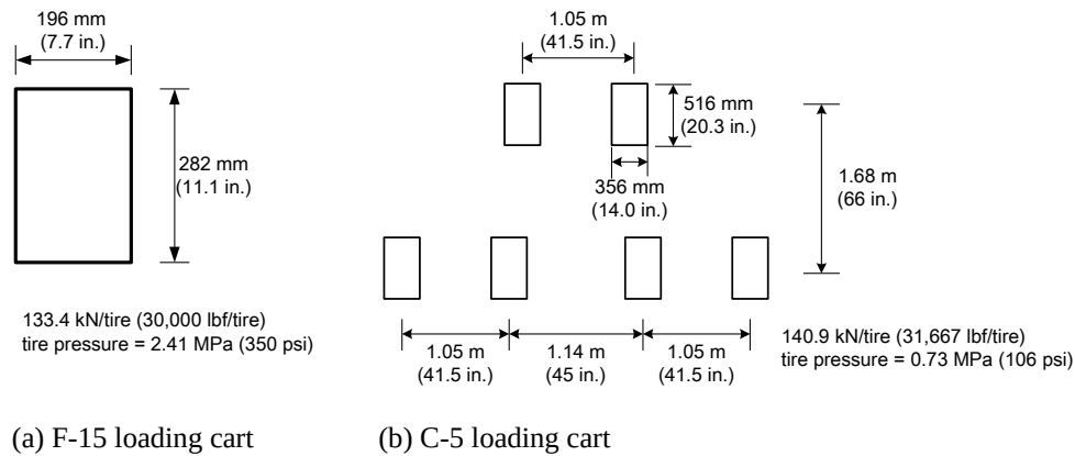
Figure 5. Footprint of single cartload for stress analysis
