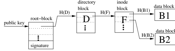
Figure 7: A simple CFS file system structure example. The root-block is identified by a public key and signed by the corresponding private key. The other blocks are identified by cryptographic hashes of their contents.
