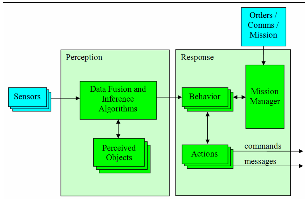
Figure 2.4. Behavioral Autonomous Vehicle Control as Implemented in the Pennsylvania State University Applied Research Laboratory Intelligent Control Architecture (After: Lewis and Weiss, 04)
