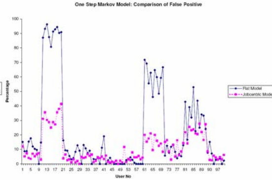
(b) Markov Model - False Positive Rate
