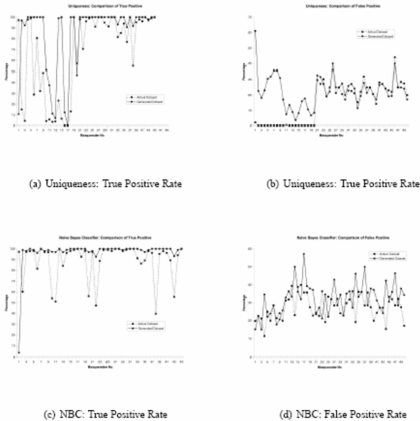
Figure 15: True positive & false positive rates 1v49 for both actual and generated data sets
