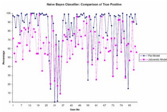
(c) Naive Bayes Model - True Positive Rate
