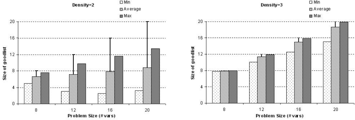
Figure 2.6: OptAPO centralization as measured by goodlist size. We display the minimum, maximum, and average amount of centralization of all the agents in a problem. The upper line above each bar marks n (# of variables), which is the maximum possible centralization at each problem size. Each measurement is the average of 50 problems.
