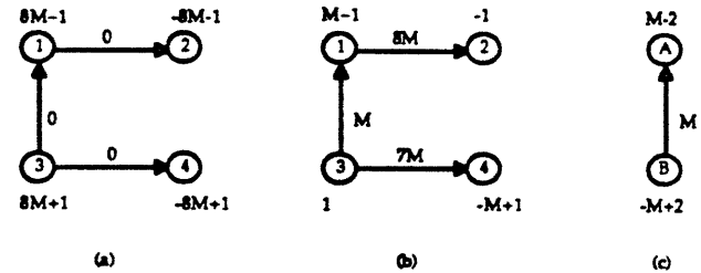
FIGURE 2. A PATHOLOGICAL EXAMPLE FOR THE RHS-SCALING ALGORITHM
