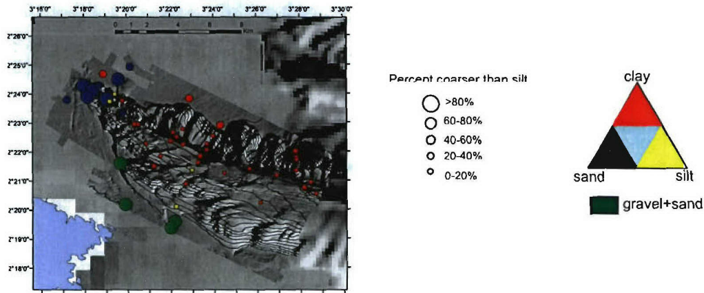
Figure 3. Surficial grain size in Cap de Creus canyon. Note the much coarser grained sediment on the southern flank compared to the northern.
