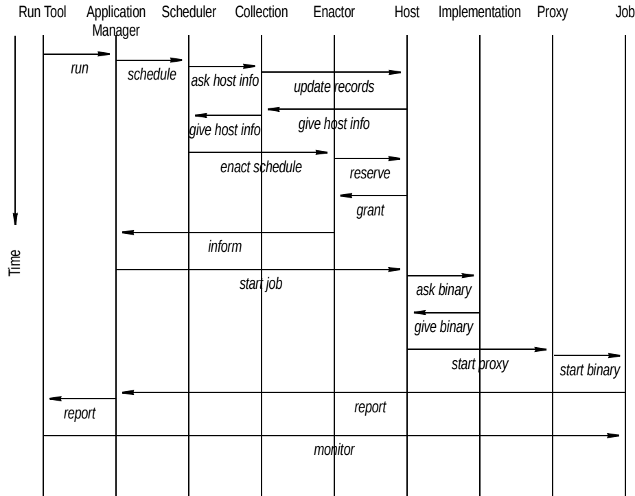
Figure 1. Scheduling Process in Legion
