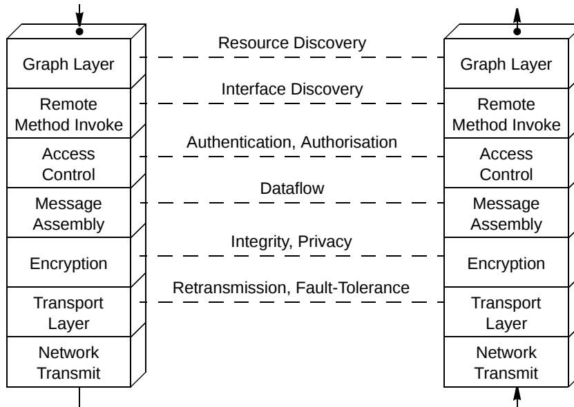
Figure 2. Protocol Stack in Legion
