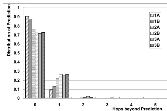
Figure 9. The Prediction of Hop Count
