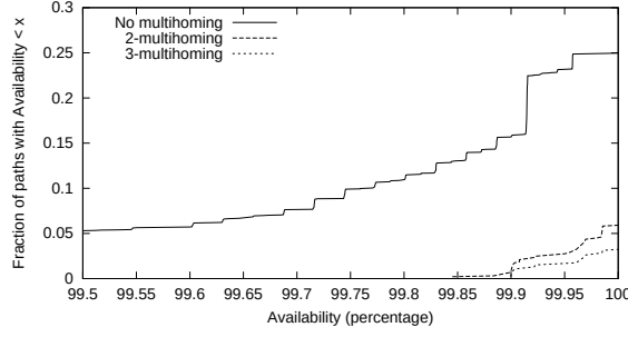
Figure 4.14: End-to-end failures: Distribution of the availability on the end-to-end paths, with and without multihoming. The ISPs in the 2- and 3-multihoming cases are the best 2 and 3 ISPs in each city based on RTT performance, respectively.
