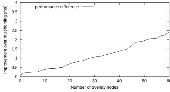
Figure 5.12: Impact of overlay network size on round-trip performance: This graph shows the mean difference between 3-overlays and 3-multihoming as overlay nodes are added.
