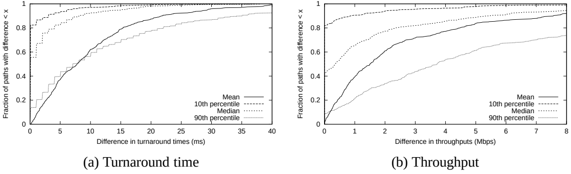
Figure 4.10: Underlying distributions: Figure showing the mean, median, 10th percentile and 90th percentile difference across various source-destination pairs. Figure (a) plots RTT, while figure (b) plots throughput (pessimistic estimate).
