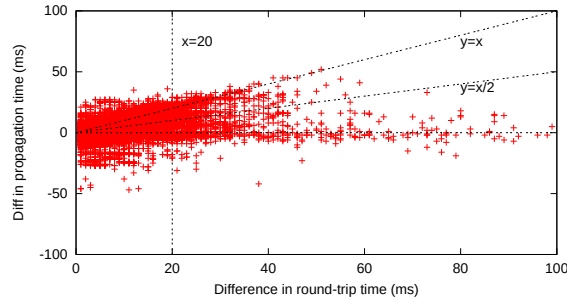
Figure 5.9: Propagation vs congestion: A scatter plot of the RTT improvement (x-axis) vs propagation time improvement (y-axis) of the indirect overlay paths over the direct paths.
