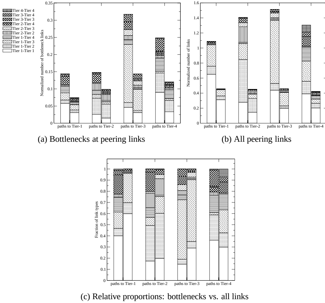
Figure 3.8: Relative prevalence of peering bottlenecks: Graph (a) shows the average number of bottlenecks of each kind appearing between ISPs, classified by path type. The graph in (b) shows the total number of links (bottleneck or not) of each kind appearing in all the paths we considered. In (a) and (b), the left bar shows the overall average number of links, while the right shows the average number of unique links. Graph (c) shows relative fraction of peering bottlenecks of various types (left bar) and the average path composition for all links (right bar).
