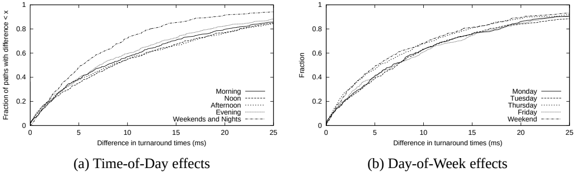
Figure 4.11: Time of day effects: Figures plotting the impact of the time-of-day (Figure (a)) and day-of-week (pessimistic, Figure (b)) on RTT performance. All times are in EDT.
