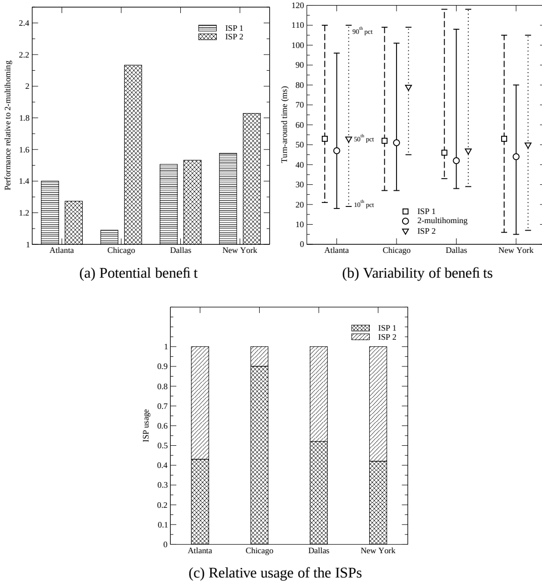
Figure 4.6: 2-multihoming evaluation: The average benefits are shown in (a). Graph (b) shows the median, 10th and 90th percentile turnaround times for each ISP and for 2-multihoming. The relative usage of the two ISPs in the optimal schedule is shown in (c).
