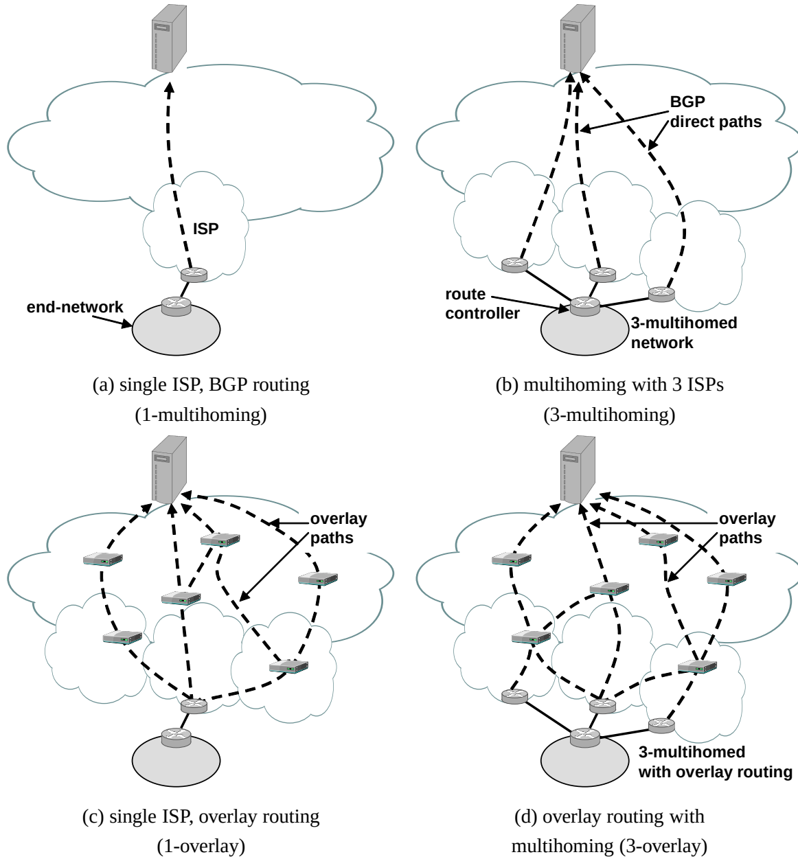
Figure 5.1: Routing configurations: Figures (a) and (b) show 1-multihoming and 3-multihoming, respectively. Corresponding overlay configurations are shown in (c) and (d), respectively.
