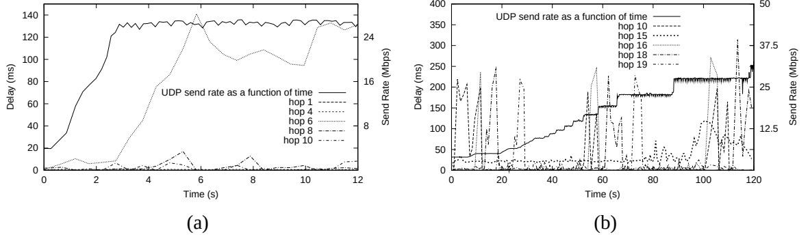
Figure 3.4: The operation of BFind: In either graph, queueing delay is shown on the left y-axis. The instantaneous UDP rate is shown on the right y-axis. In (a), BFind identifies hop 6 as the bottleneck. In (b), BFind identifies hop 15 as the bottleneck, although this could potentially be a false positive.
