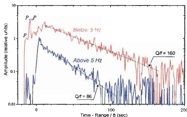
Figure 2. Amplitude-time decay for Lg coda from PNE QUARTZ-4, measured near the position of PNE QUARTZ-2 (Figure 1 Error! Reference source not found.). Note the increasing amplitude decay rate with frequency; this increase is indicative of seismic attenuation. Q/f values measured from the slopes are given in the labels.
