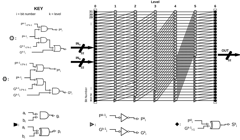
Figure 3: Brent-Kung adder
