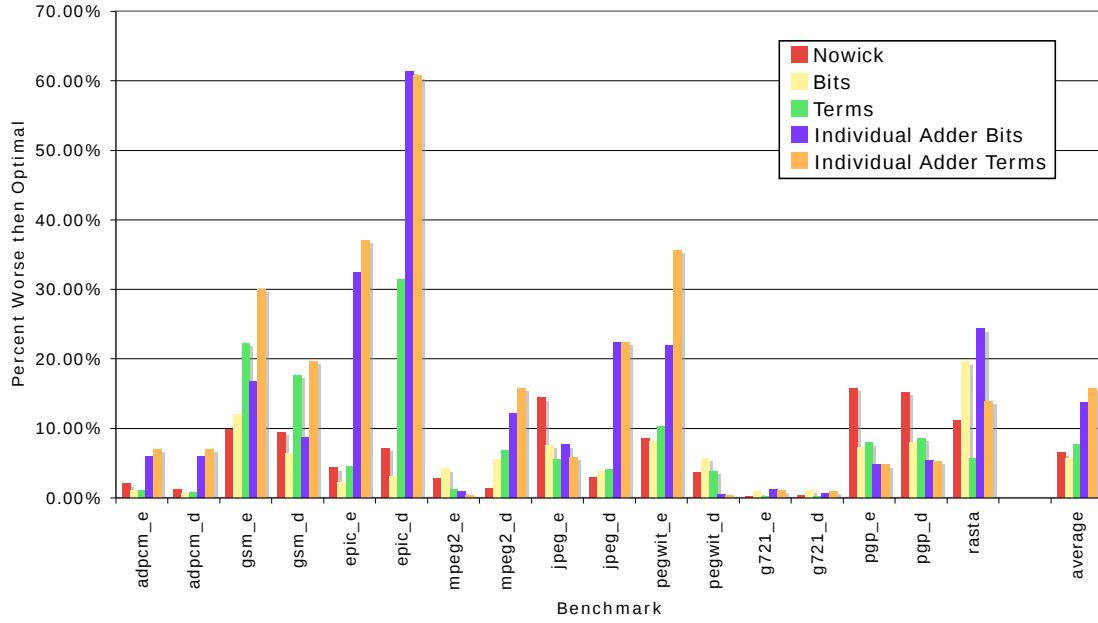
Figure 12: The percent error of various latency approximation functions when evaluated on program executions using different inputs than the profiled execution. A maximum of 35 literals per a function is allowed. In some cases, the approximation functions remain effective, but in others the error dramatically increases compared to that of Nowick.
