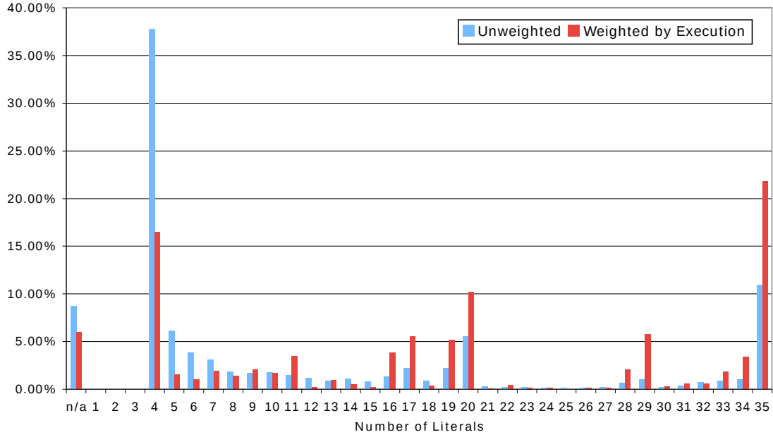
Figure 11: The distribution of the size of lateness approximation functions across all adders of all the benchmarks. The unweighted distribution counts each adder equally whereas the weighted distribution weights each adder by its execution frequency. Adders which do not demonstrate detectable early termination behavior frequently enough to benefit from early termination fall in the n/a category.
