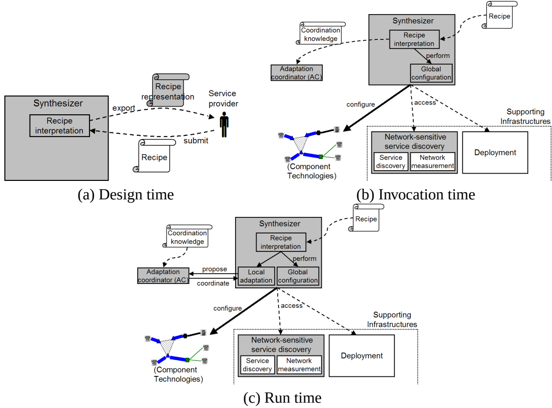
Figure 2.6: Operations of a recipe-based self-configuring service.
