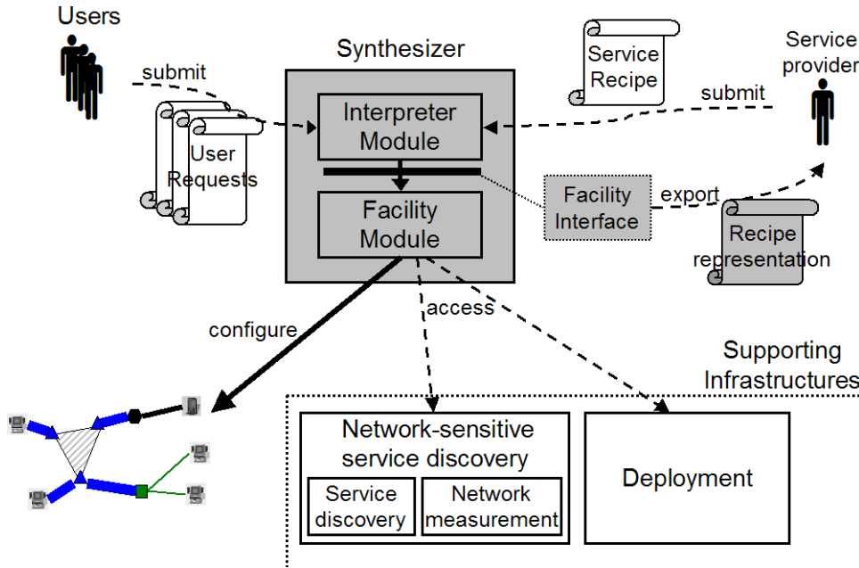
Figure 4.1: Synthesizer architecture.
