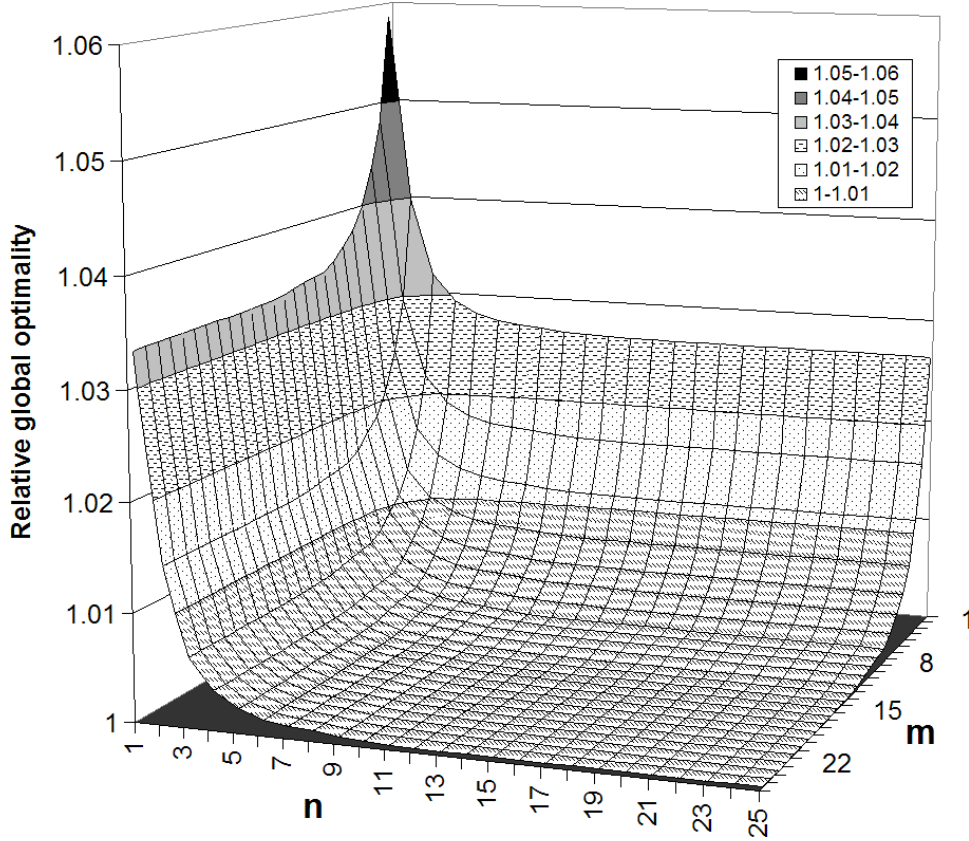
Figure 3.21: Relative global optimality for unweighted-25.
