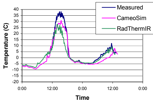
Figure 6 Comparisons of RadThermIR and CAMEO-SIM simulations for the foil panel's physical surface temperature.
