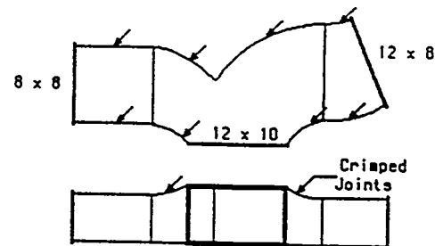
Figure IV-6 Example of Commercial Vent (0.025" Galvanized Steel) with Out-of-Plane Crimped Joints
