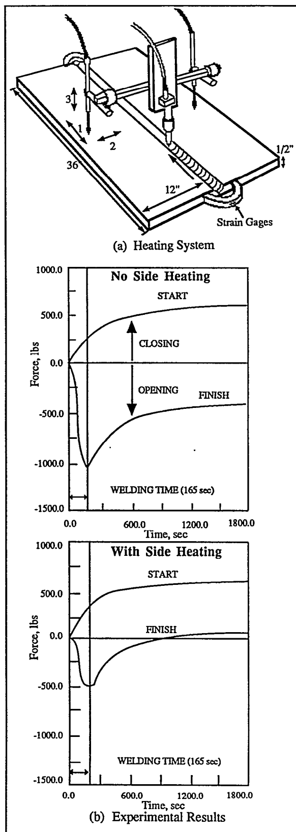
Figure 5 Reduction of Forces Acting on the Rings Attached to Starting and Finishing Ends of a Butt Weld
